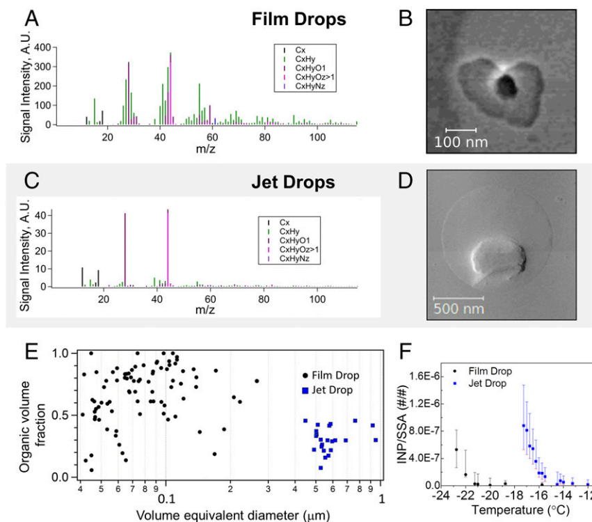
Fig. 3. Differences in chemical composition between submicrometer film drop and jet drop particles: AMS mass spectra for submicrometer (A) film and (C) jet drop particles. Typical AFM phase images for submicrometer (B) film drop particles and (D) jet drop particles. (Scale bars: B, 100 nm long; D, 500 nm long.) (E) Organic volume fractions for submicrometer particles produced by film and jet drops (determined from AFM images). (F) Number fraction of INPs in film and jet drop particles. Error bars represent 1 SD.
