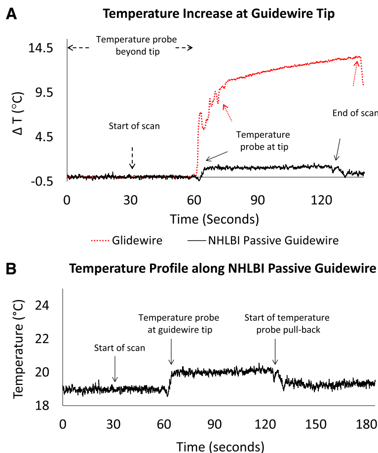
Fig. 5 In vitro temperature measurements. a Temperature at the tip of the NHLBI passive guidewire (black) and the commercial Glidewire comparator (red) during 60 s bSSFP CMR scans at a flip angle of 75°. b Pullback of the temperature probe alongside the NHLBI passive guidewire. After baseline steady state, scanning begins (at t = 30 s), then the probe is withdrawn from beyond the guidewire tip back to the guidewire tip (at t = 60 s). The probe remains at the tip, during which time the temperature rises by 1.2 °C. Finally the probe is pulled back further (beginning at t = 120 s) indicating that the temperature rise is confined to the tip
