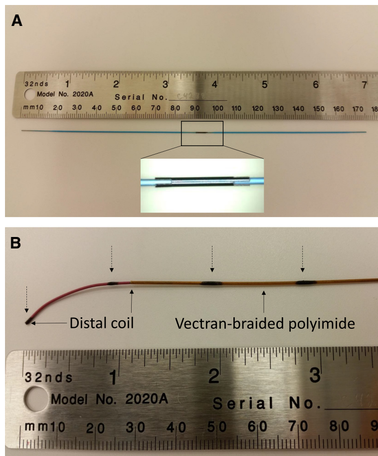
Fig. 2 Components of the NHLBI passive guidewire. a This photograph shows two Pebox-coated nitinol segments are joined by a nitinol connector. b The distal tip incorporates a non-resonating coil for mechanical flexion, which is wrapped over the shaped and tapered nitinol rod segment. The distal and proximal ends of the coil are indicated by arrows. Iron oxide markers (dashed arrows) are painted over the tip coil and the Vectran-braided polyimide tubing prior to the application of the final polymer jacketing layer
