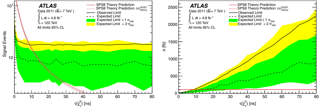
FIG. 7 (color online). 95% C.L. limits on (left) the number of signal events and (right) the SPS8 signal cross section, as a function of NLSP lifetime, for the case of \Lambda = 120 TeV. The region below the limit curve is excluded at 95% C.L.
