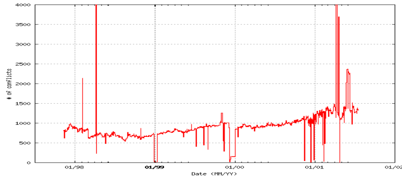
Fig. 2. OASC events in the Internet from 1998 to 2001
