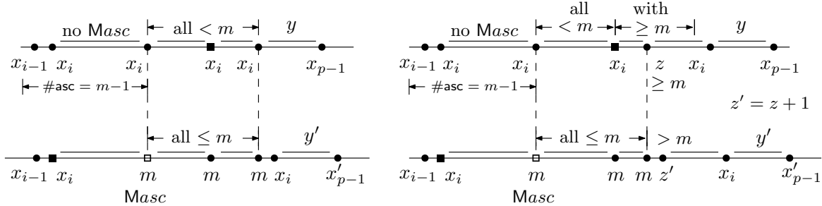
Figure 8.7: Case 2: the rightmost x_{i-1} is next to x_i and no Masc appears between the first two x_i 's that are after x_{i-1} . Here x_i = \text{Rmin}(s)_i with i = \text{rpos}(s) and y' = y + 1 if y \geq m ; otherwise y' = y .
