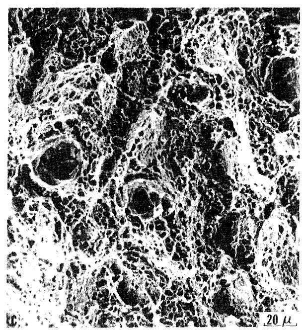
Fig. 83. A and B 4330 (1200, IBQLN) 350 C 4300 (870, OI1) 350
