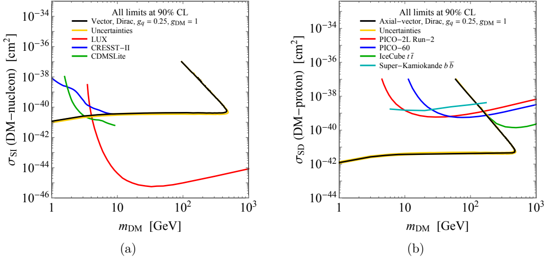
Figure 2: A comparison of LHC results to the m_{\text{DM}}\text{-}\sigma_{\text{SI}} (a) and m_{\text{DM}}\text{-}\sigma_{\text{SD}} (b) planes. Unlike in the mass-mass plane, the limits are shown at 90% CL. The LHC contour in the SI (SD) plane is for a vector (axial-vector) mediator, Dirac DM and couplings g_q = 0.25 and g_{\text{DM}} = 1 . The LHC SI exclusion contour is compared with the LUX, CDMSLite and CRESST-II limits, which are the most constraining in the shown mass range. The SD exclusion contour constrains the DM-proton cross section and is compared with limits from the PICO experiments, the IceCube limit for the t\bar{t} annihilation channel and the Super-Kamiokande limit for the b\bar{b} annihilation channel. The depicted LHC results are intended for illustration only and are not based on real data.
