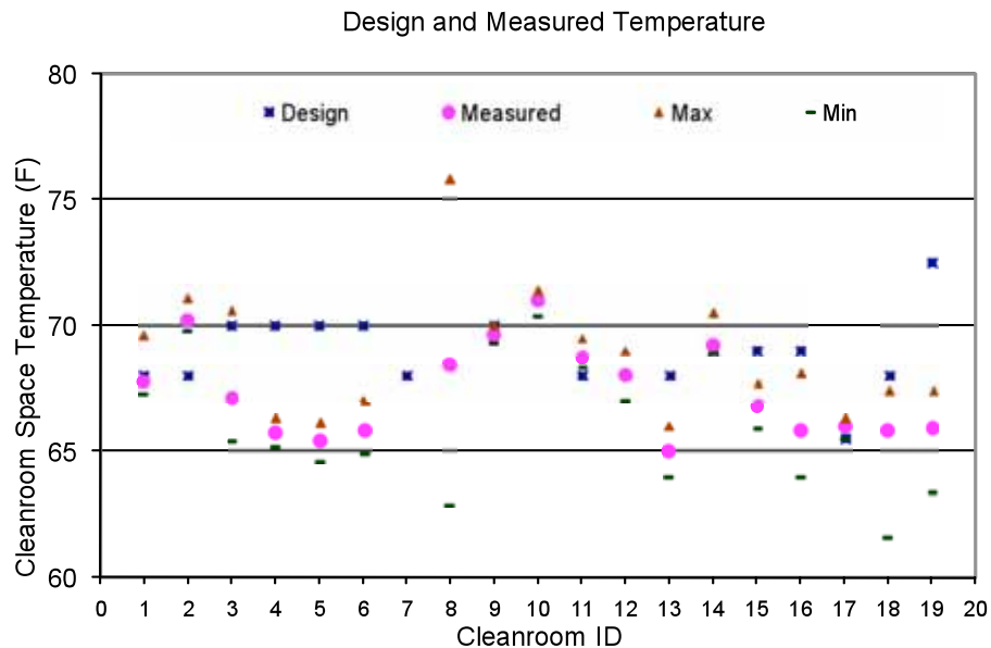
Figure 1. Design and measured temperature ranges for cleanrooms in the LBNL database
