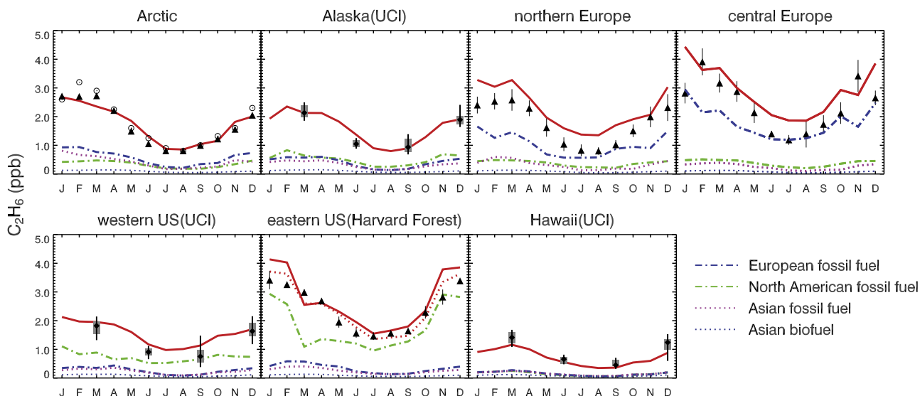
Figure 3a. Surface air C 2 H 6 mixing ratios for the sites in Figure 1. Model values (red lines) are compared to observations (black). For UCI data, the diamonds are monthly medians, with points outside the median ±2σ excluded; the 25th and 75th percentiles (boxes) and 10th and 90th percentiles (vertical bars) are also shown. Arctic data are from Alert (open circle) and Zeppelin (solid triangle). Observations for other regions are monthly means (black triangle) ± 1 standard deviation. Model results with optimized North American sources on the basis of the INTEX-A aircraft data (section 5) are shown for Harvard Forest (red dotted) and not for other sites where differences with the standard simulation are negligible. Also shown as dashed and dotted lines are contributions from major source types and regions to the model C 2 H 6 .
