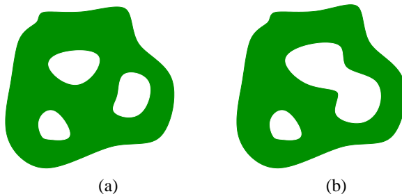
Fig. 1: Two semiclassical phase space distributions of fermions, related by a topological transition that changes the number of components of the Fermi surface by \pm 1 .
