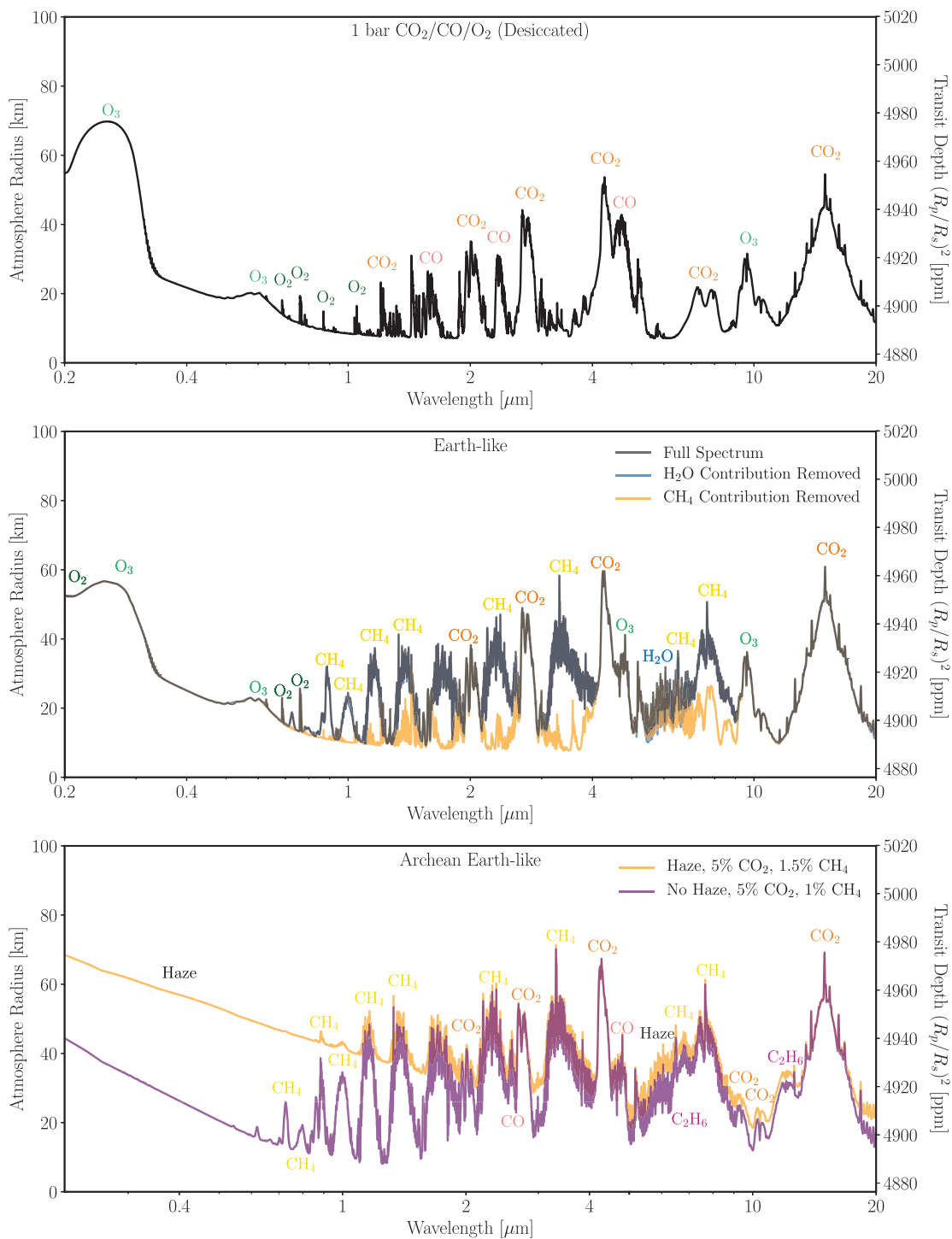
FIG. 20. Similar to the transmission spectra of Fig. 17, but the top panel is for the heavily H-depleted \text{CO}_2/\text{O}_2/\text{CO} atmosphere in photochemical equilibrium from Section 4.2.2.3 (also see Gao et al. , 2015). Note the strong CO bands at 2.35 and 4.6 \mu\text{m} compared to other cases. The middle panel shows the photochemically self-consistent modern Earth (black) with preindustrial biological fluxes of \text{CH}_4 , CO, and \text{N}_2\text{O} orbiting Proxima Centauri b. It also shows Earth’s spectrum with \text{CH}_4 (orange) and \text{H}_2\text{O} (blue) removed, to show the relative contributions of each to the spectrum. The weak \text{H}_2\text{O} features result from transmission probing higher, drier altitudes down to about 10 km, but water being mostly concentrated in the lower portion of the troposphere, below \sim 12 km. In addition to their intrinsic weakness, the \text{H}_2\text{O} features are also swamped by \text{CH}_4 absorption, which also raises the effective tangent height to drier altitudes. The bottom panel shows the Archean Earth-like planets with (orange) and without (purple) organic haze orbiting Proxima Centauri. A haze absorption feature is present near 6 \mu\text{m} , and haze produces the spectral slope continuing into the NIR for the hazy spectrum.
