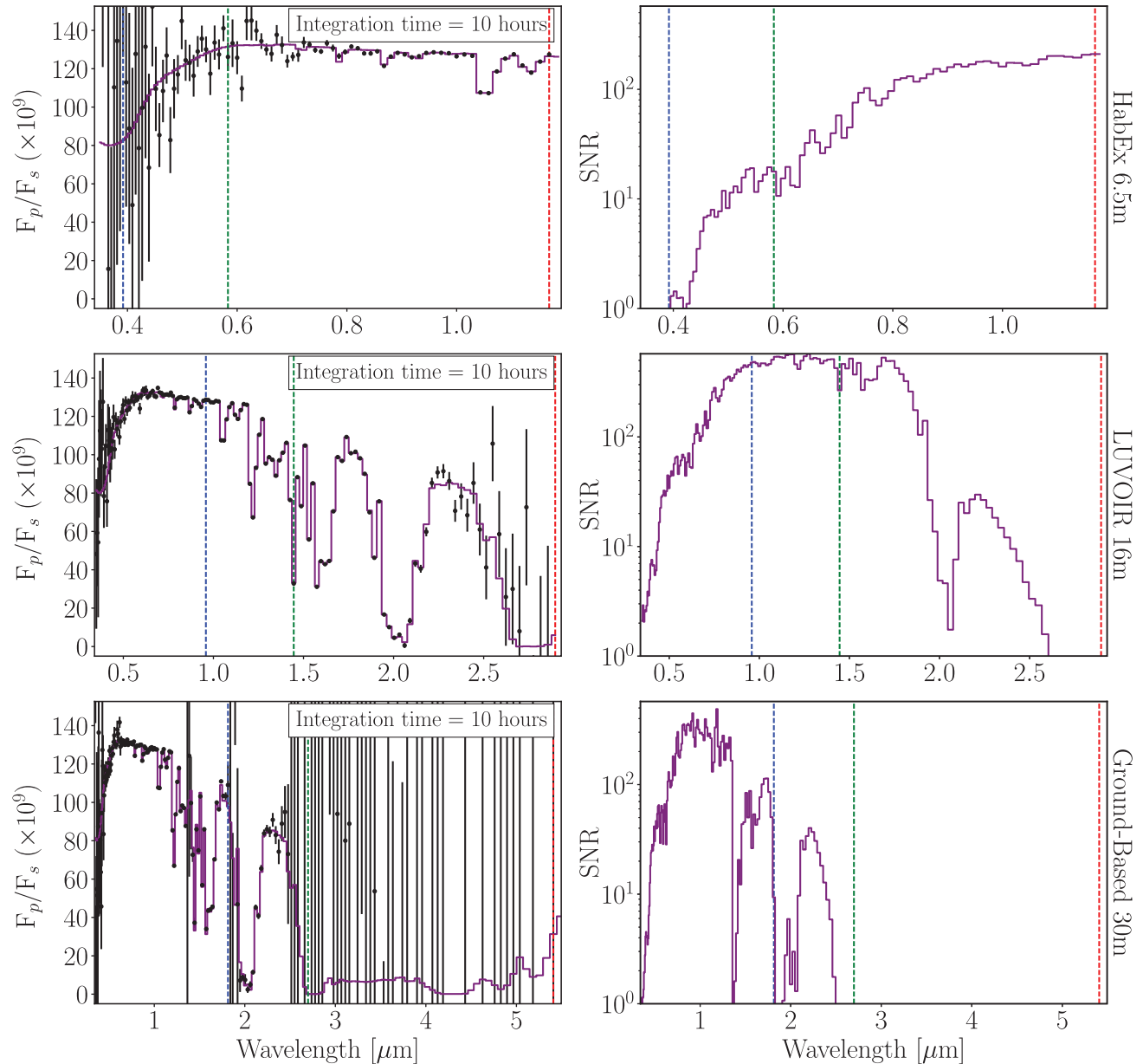
FIG. 23. Similar to the coronagraph simulations of Fig. 21, but for the 90 bar cloud-covered Venus-like planet.
