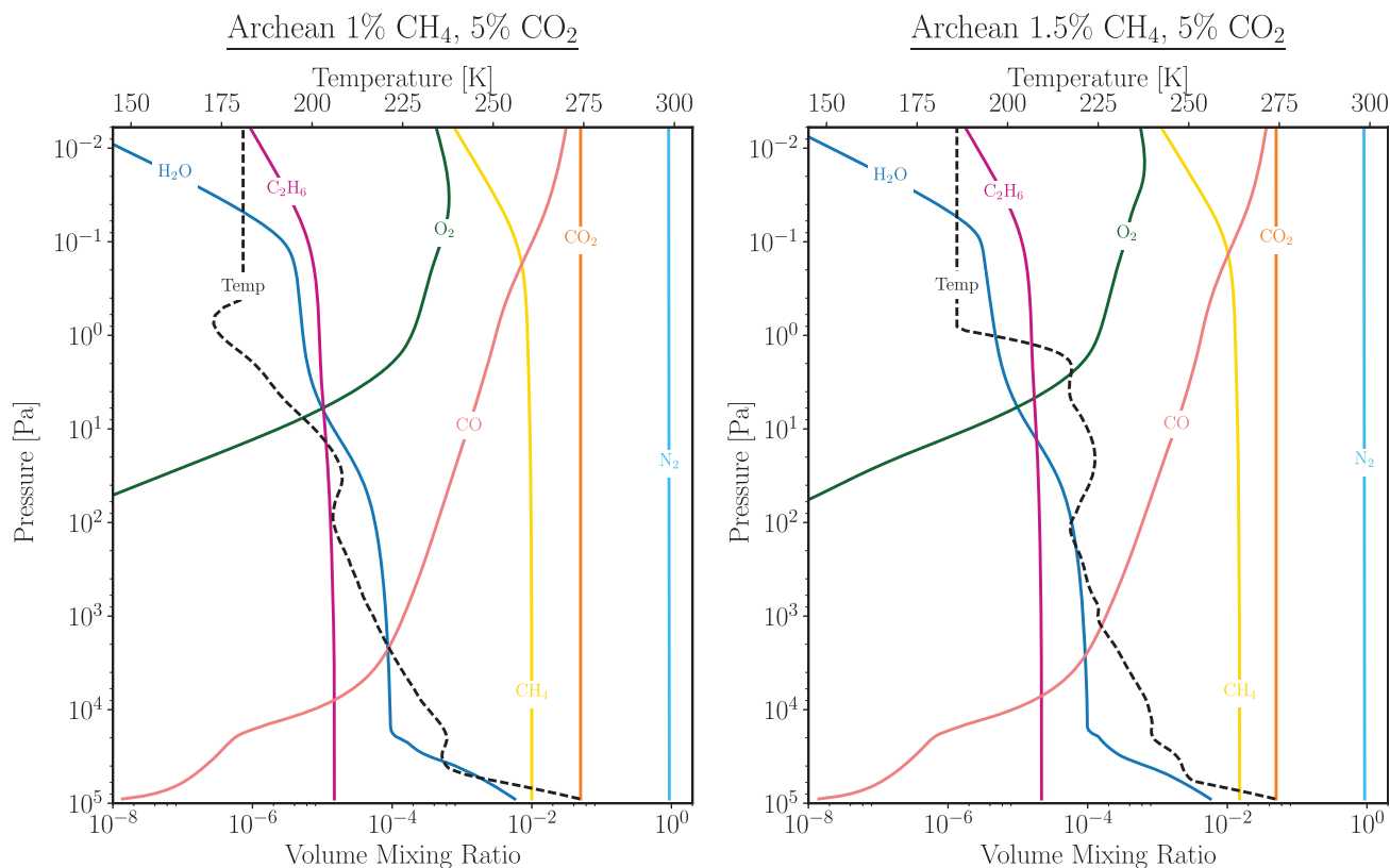
FIG. 9. Temperature (top x axes; black dashed) and gas mixing ratio profiles (bottom x axes) for Archean analog planets orbiting Proxima Cen b. The moderate temperature inversion seen in the right (1.5% CH 4 ) plot is due to UV absorption by the haze. UV shielding by the haze in the 1.5% CH 4 plot (right) prevents photolysis of gases such as methane and ethane at higher altitudes than in the 1% CH 4 plot (left). Note the temperature profile becomes an isoprofile above the top of the climate model grid when passed into the photochemical model.
