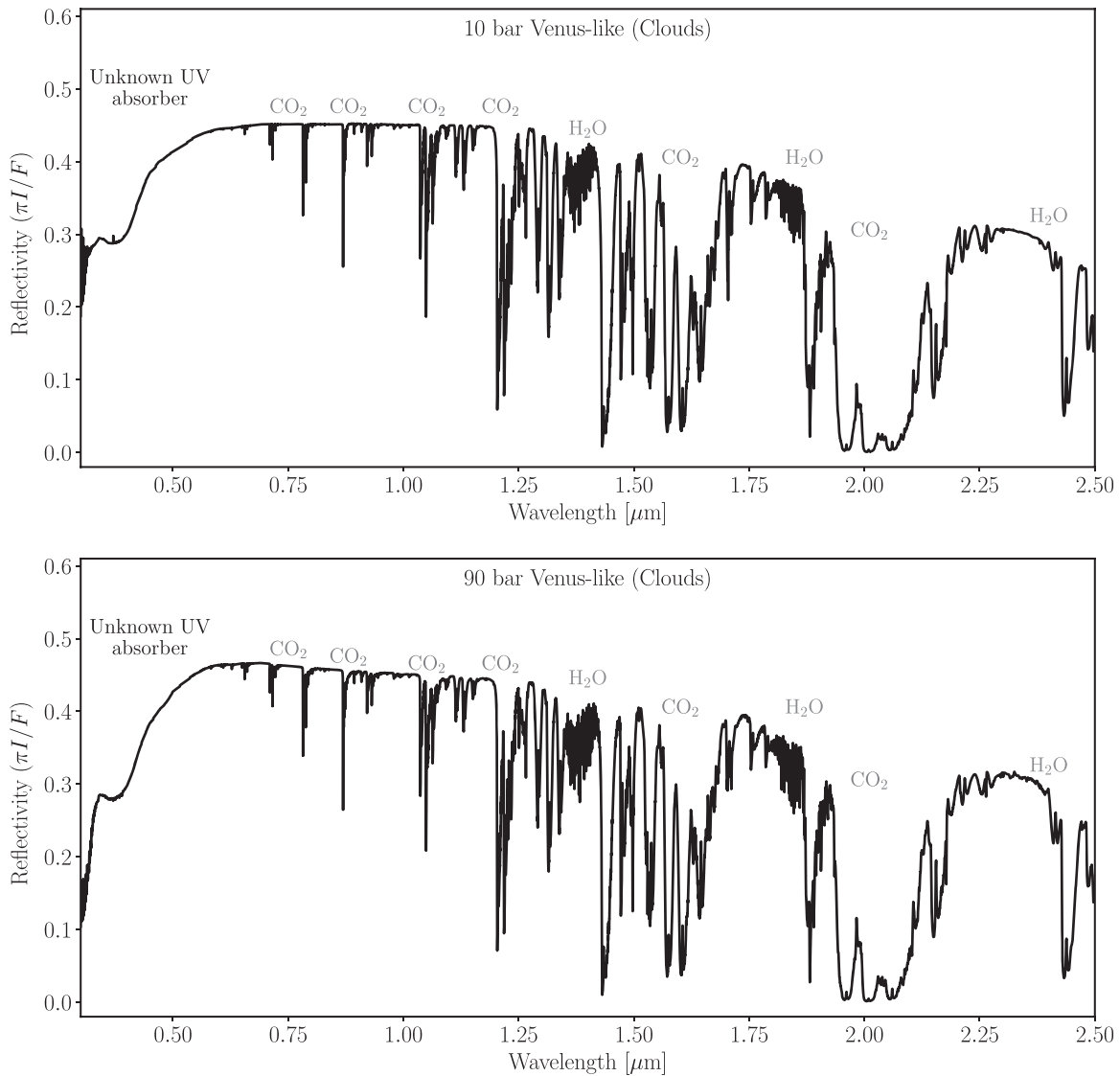
FIG. 14. Similar to the reflected light spectra of Fig. 12, but for the Venus-like worlds with 10 bar (top) and 90 bar (bottom) \text{CO}_2 atmospheres. Strong \text{CO}_2 absorption features are present at several wavelengths. The two spectra are similar because the cloud decks in both atmospheres occur at roughly the same pressure, so about the same amount of total atmosphere is sensed in each spectrum.
