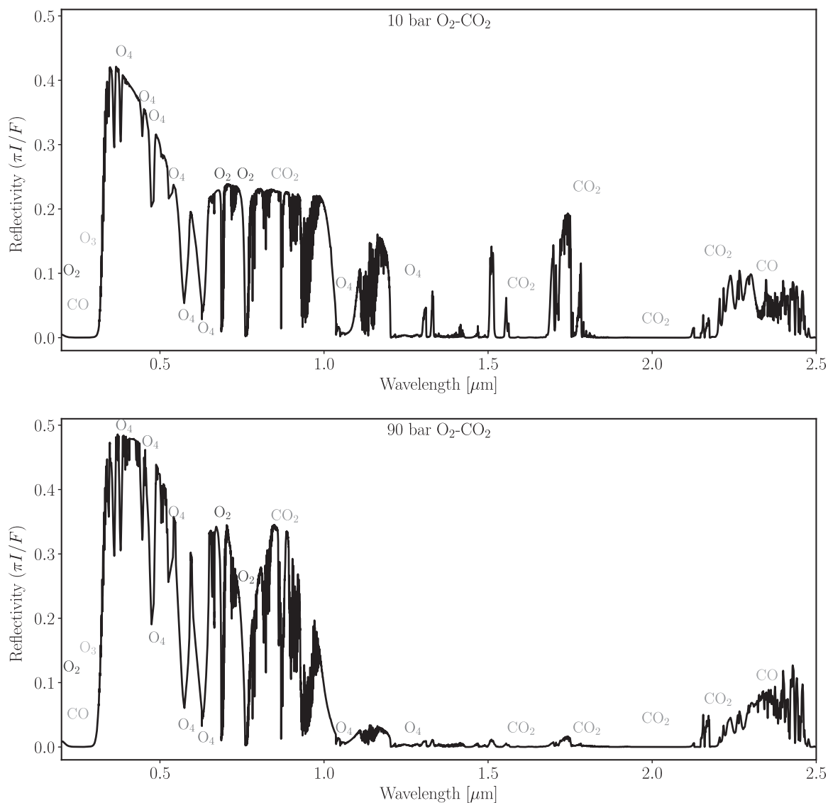
FIG. 13. Similar to the reflected light spectra of Fig. 12, but for the clear O 2 -CO 2 (45% O 2 , 45% CO 2 , 10% N 2 , 20 ppm H 2 O) atmospheres with surface pressures of 10 bar (top) and 90 bar (bottom) for comparison with O 2 -only and Venus cases.
