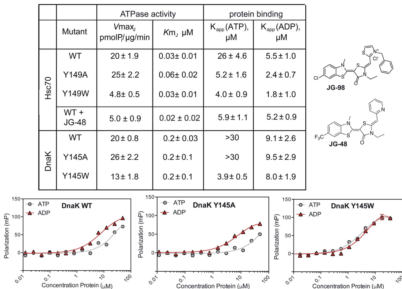
Fig. 2 Y149W and Y145W partially mimic the biochemical behavior of inhibitor treatment. Summary of ATPase activity and peptide-binding assays, using purified human Hsc70 or E. coli DnaK and the corresponding mutants. Steady state ATPase activity was measured using malachite green (MG) and binding to a fluorescent FAM-HLA tracer was measured using fluorescence polarization (FP). In the ATPase assays, a J-domain protein (JDP; either DnaJA2 or DnaJ) was added to increase signal intensity. Examples of the FP results for DnaK and its mutants are shown (bottom). Error bars represent SEM of two independent, biological replicates, each performed in technical triplicate. See the Methods for details.
