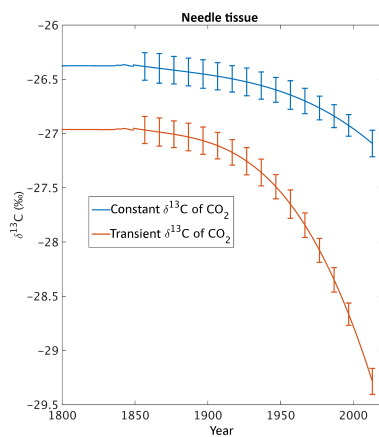
Figure 6. Simulation of \delta^{13}\text{C} of needle tissue using the limited nitrogen (default) CLM run. In the constant \delta^{13}\text{C} of \text{CO}_2 ( \delta_{\text{atm}} ) simulation the model boundary condition was -6\text{‰} , whereas the transient \delta_{\text{atm}} simulation varied over time (Fig. 2).
