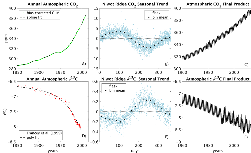
Figure 2. Niwot Ridge synthetic data product for atmospheric \text{CO}_2 concentration ( c_a ) (a, b, c) and \delta^{13}\text{C} of \text{CO}_2 ( \delta_{\text{atm}} ) (d, e, f). The final time series (c, f) were used as a boundary condition for CLM, and created by combining the annual trends reported by Francey et al. (1999) adjusted for Niwot Ridge (a, d) with the mean seasonal cycles measured at Niwot Ridge (b, e).
