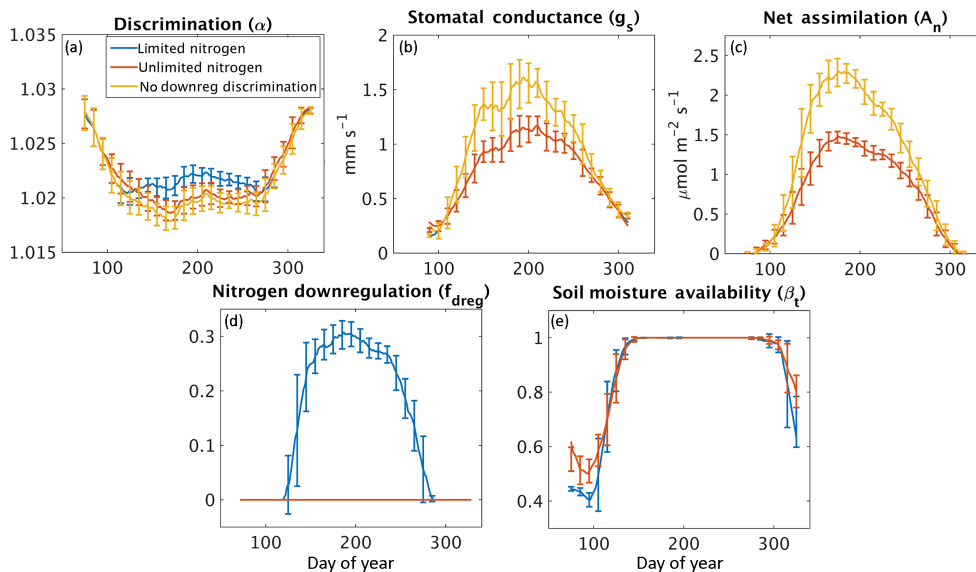
Figure 9. The seasonal pattern of discrimination (a) and diagnostic variables that explain the discrimination pattern in Fig. 8. The individual tiles provide behavior for days 75–325 for (a) \alpha , (b) g_s , (c) A_n , (d) f_{\text{dreg}} , and (e) \beta_t . Where the no-downregulation discrimination model simulation is not shown, it is identical to the limited nitrogen simulation. Uncertainty bars represent 95 % confidence intervals of interannual variation from 2006 to 2012.
