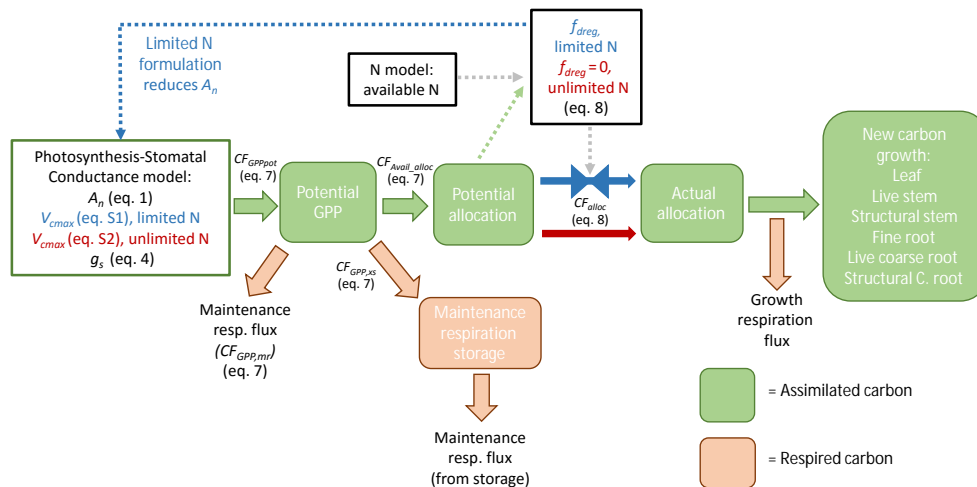
Figure 1. A simplified representation within CLM4.5 of assimilation and allocation of carbon for conifer species. The colored boxes and solid arrows represent carbon pools and carbon fluxes, respectively. The clear background boxes represent CLM submodels. N limitation is applied if the available N cannot meet the demand determined by the available carbon for allocation ( CF_{avail\_alloc} ) and the C : N biomass ratio. The blue and red text and arrows represent the limited and unlimited nitrogen formulations, respectively. The no-downregulation discrimination formulation is exactly the same as the limited N formulation in this schematic.
