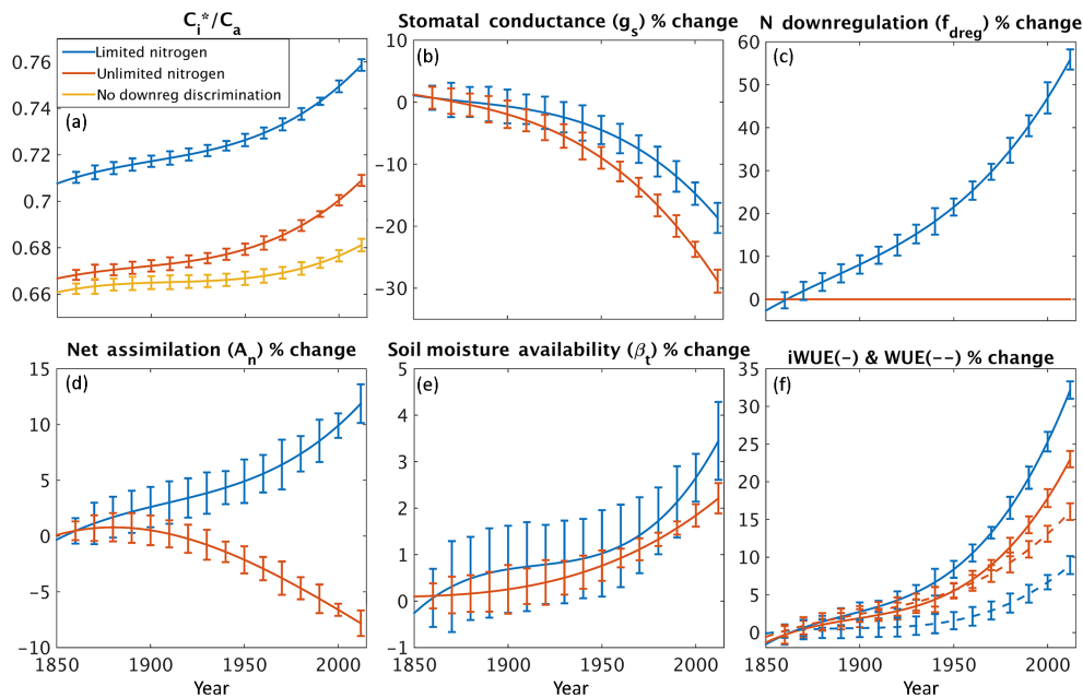
Figure 7. Diagnostic model variables that explain the discrimination trends (Fig. 5) for the three model formulations as described in Table 2 for (a) c_i^*/c_a , (b) g_s , (c) f_{dreg} , (d) A_n , (e) \beta_t , and (f) the WUE and iWUE. Where the no-downregulation discrimination simulation is not shown, it was identical to the limited nitrogen simulation. Uncertainty bars represent 95 % confidence intervals of diagnostic variable variation as a result of cycling the site-level meteorology observations. The dashed lines represent WUE and the solid lines represent iWUE in (f).
