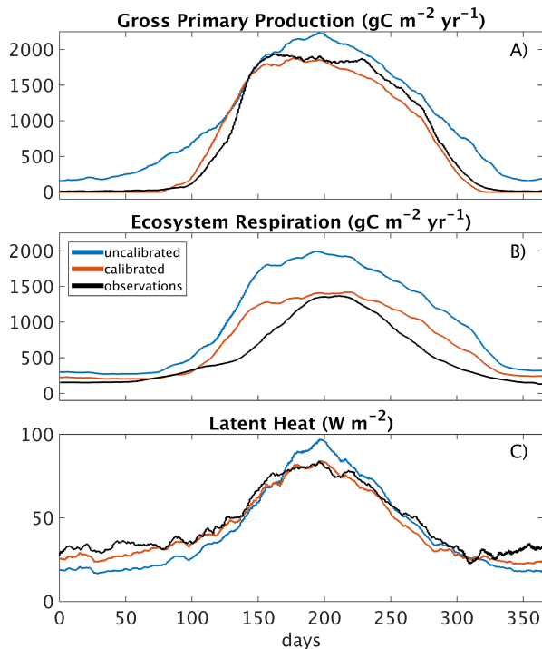
Figure 3. Seasonal averages (1999–2013) of simulated and observed land–atmosphere fluxes for (a) gross primary production (GPP), (b) ecosystem respiration (ER), and (c) latent heat (LE) for the limited nitrogen simulation. The observations are taken from the Ameriflux L2 processed eddy covariance flux tower data, partitioned into GPP and ER using the method of Reichstein et al. (2005). The uncalibrated simulation represents the CLM simulation without V_{\text{cmax}} scaling and the calibrated simulation represents the CLM run using the V_{\text{cmax}} scaling approach.
