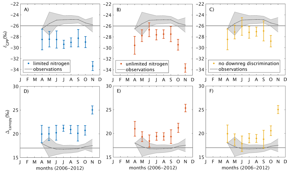
Figure 8. The seasonal pattern of photosynthetic discrimination as shown through \delta_{\text{GPP}} (a, b, c) and \Delta_{\text{canopy}} (d, e, f). Uncertainty bars represent 95 % confidence bounds of simulated monthly average values from 2006 to 2012. Gray-shaded observation bounds represent 95 % confidence intervals of observed monthly average values based upon isotopic mixing model using Reichstein et al. (2005) partitioning of net ecosystem exchange flux described by Bowling et al. (2014). The horizontal lines at \delta^{13}\text{C} of -26\text{‰} (a, b, c) and 17\text{‰} (d, e, f) are included for reference.
