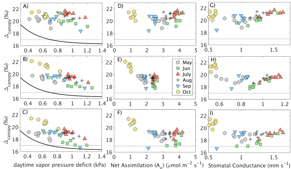
Figure 10. Relationship between monthly average photosynthetic discrimination and monthly average vapor pressure deficit (a, b, c), A_n (d, e, f) and g_s (g, h, i) from 2006 to 2012. The rows represent the limited nitrogen (a, d, g), unlimited nitrogen (b, e, h), and no-downregulation discrimination (c, f, i) simulations. The black lines in (a), (b) and (c) are based on an exponential fitted line from the observed relationship at Niwot Ridge (Bowling et al., 2014). The horizontal lines represent \delta^{13}\text{C} of 17‰ and are included for reference.
