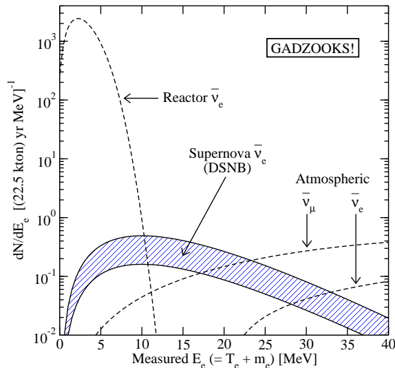
Figure 2. The expected coincident signals in Super-K with 100 t GdCl 3 . Detector energy resolution is properly taken into account. The upper supernova curve is the current SK relic limit, while the lower curve is the theoretical lower bound.
