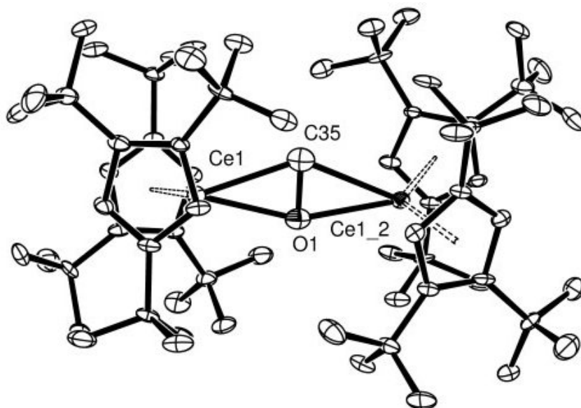
Figure 3. ORTEP diagram for [(1,2,4-(\text{Me}_3\text{C})_3\text{C}_5\text{H}_2)_2\text{Ce}]_2(\mu\text{-OCH}_2) , 2 . (50% probability ellipsoids); the toluene of crystallization is not shown. The non-hydrogen atoms except C(35) were refined anisotropically and the hydrogen atoms were placed (but not shown) in calculated positions. Ce(1)-C(ave) = 2.86 \pm 0.05 Å, Ce-Cp'(ring perpendicular) = 2.59 Å (ave.) Ce(1)-O(1) = 2.443(2) Å, Ce(1)-C(35) = 2.554(4) Å, C(35)-O(1) = 1.39(1) Å, C(35)-Ce(1)-O(1) = 32.2(3)^\circ Cp'(ring perpendicular)-Ce-Cp'(ring perpendicular) = 135^\circ .
