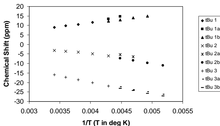
Figure 4. Chemical Shift vs. 1/T for (Cp' 2 Ce) 2 (μ-OCH 2 ) ( 2 ).
