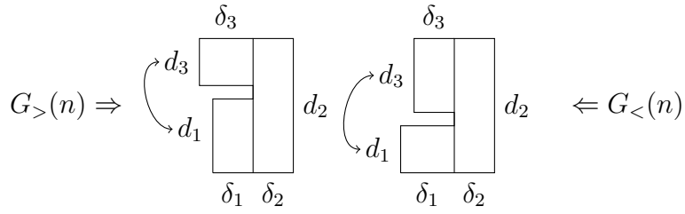
Figure 7.10: Solutions to (*) counted by G_<(n) are equinumerous with solutions to (*) counted by G_>(n) .
