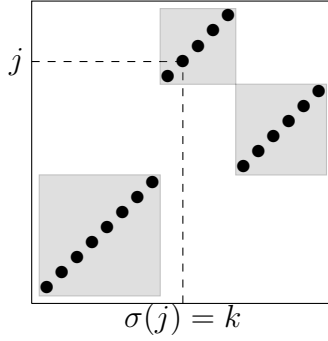
Figure 3.7: Random \sigma \in \mathcal{S}_{19}(A^{(4)})
