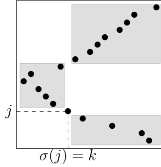
Figure 3.3: Random \sigma \in \mathcal{S}_{19}(A^{(2)})
