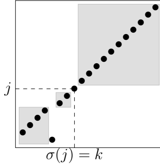
Figure 4.2: Random \sigma \in \mathcal{S}_{19}(B^{(2)})
