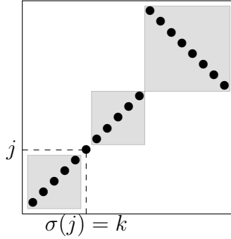
Figure 4.3: Random \sigma \in \mathcal{S}_{19}(B^{(3)})
