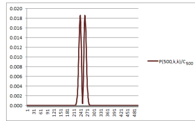
Figure 8.4: Values of P_{500}(k, k) .
