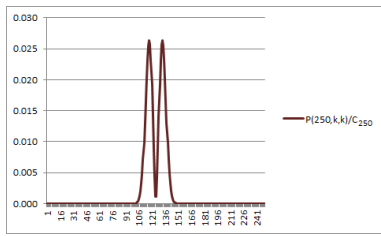
Figure 8.3: Values of P_{250}(k, k) .
