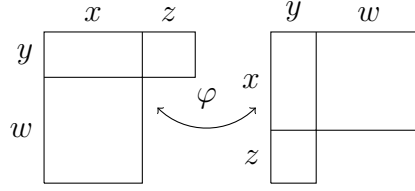
Figure 7.3: Summing y is equivalent to summing y + w - z , as shown by the above involution \varphi .
