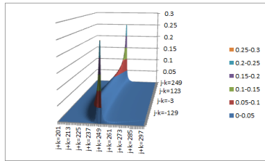
Figure 8.8: A closer look at Q_{250}(j, k) , 201 \leq j + k \leq 301 .
