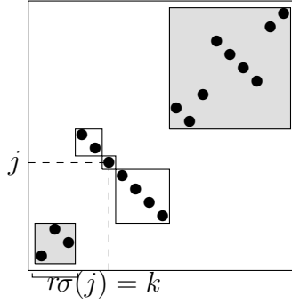
Figure 3.1: Random \sigma \in \mathcal{S}_{19}(A^{(1)})
