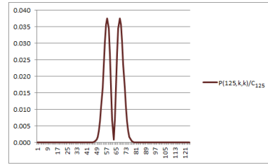
Figure 8.2: Values of P_{125}(k, k) .
