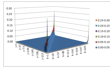
Figure 8.6: Surface of Q_{250}(j, k) .
