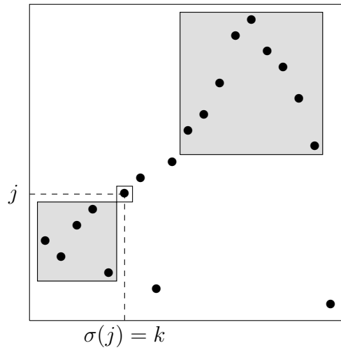
Figure 6.2: Random \sigma \in \mathcal{S}_{19}(\mathbf{132}, \mathbf{4231})
