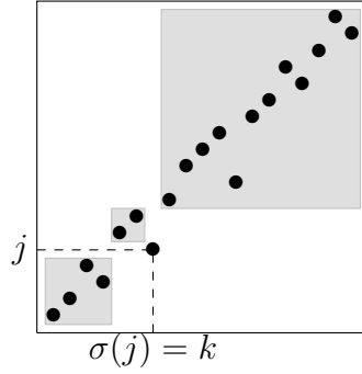
Figure 3.5: Random \sigma \in \mathcal{S}_{19}(A^{(3)})
