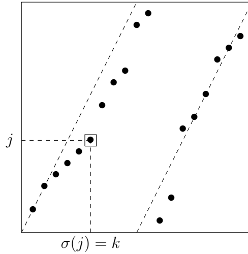
Figure 5.3: Random \sigma \in G_{19}
