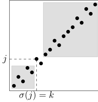
Figure 4.1: Random \sigma \in \mathcal{S}_{19}(B^{(1)})
