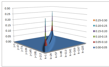
Figure 8.5: Surface of P_{250}(j, k) .
