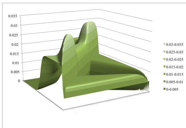
Figure 6.4: Limit shape of H_{100}(j, k) , with the corner at j = k = 100 ignored
