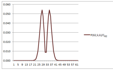
Figure 8.1: Values of P_{62}(k, k) .
