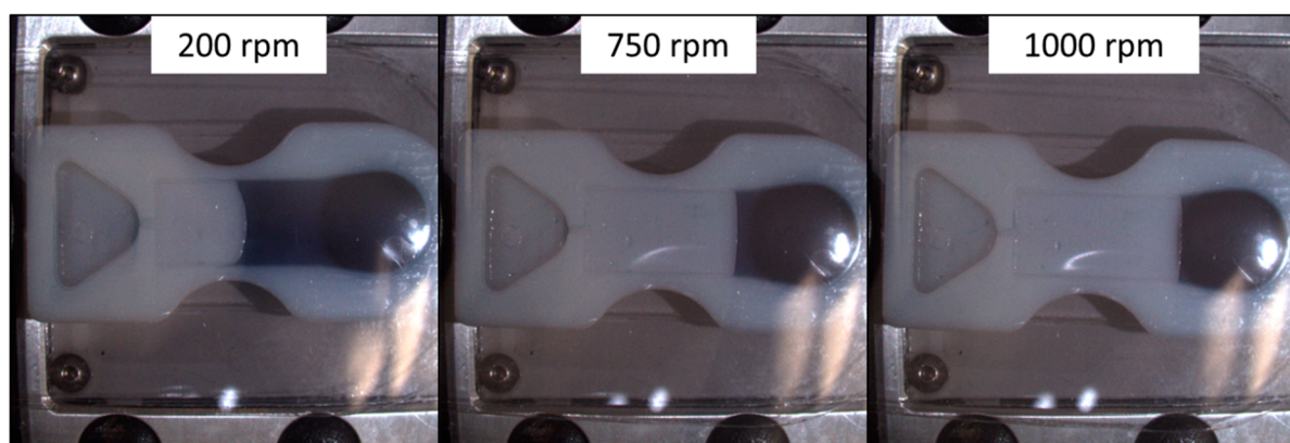
Figure 4. Fluid position in straight channel insert when spinning at 200 RPM, 750 RPM, and 1000 RPM respectively.
