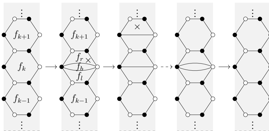
Figure 3.1: The sequence of moves in the geometric R -matrix transformation. The faces where we perform spider moves are marked by \times 's. The dashed arrow indicates a sequence of n - 1 spider moves.
