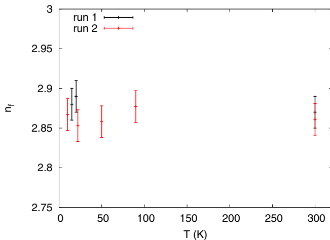
FIG. 6. Total 5f occupancy estimate n_f of URu 2 Si 2 as a function of temperature from both experimental runs. The lowest measured temperature is 10 K. No measurable temperature dependence was observed. Taking all these data together and allowing for some systematic error gives n_f = 2.87 \pm 0.08 .
