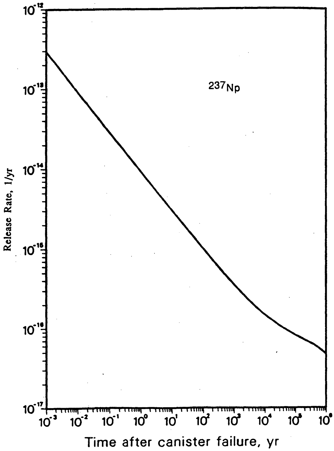
Figure 2. Release Rate of ^{237}\text{Np} by Diffusion
