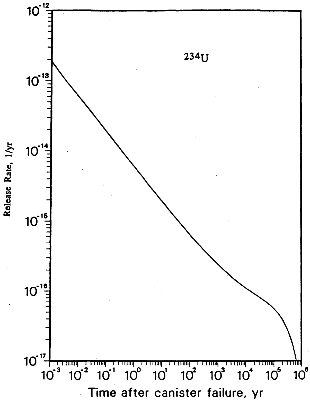
Figure 1. Release Rate of ^{234}\text{U} by Diffusion
