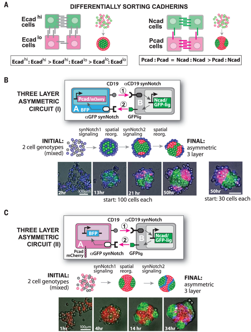
Fig. 5. Programming spherically asymmetric structures by inducing differentially sorting adhesion molecules.
