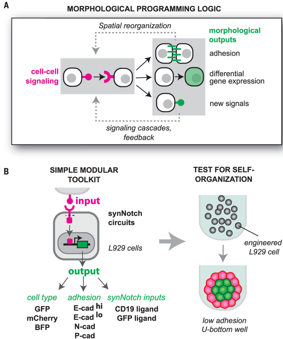
Fig. 1. Engineering cell-cell communication networks to program synthetic morphogenesis. (A) Design logic underlying our synthetic morphogenesis circuits. Engineered cell-cell signaling is used to drive changes in cell adhesion, differentiation, and production of new cell-cell signals. These outputs can subsequently be propagated to generate new cell-cell signaling relationships. (B) Molecular components used for assembly of simple morphological circuits. We used two synNotch ligand-receptor pairs (surface ligands CD19 and GFP) for cell signaling, three fluorescent proteins as markers of “differentiation,” and several cadherin molecules (expressed at different levels) as morphological outputs. Engineered circuits are transduced into L929 fibroblast cells, placed in defined numbers in low-adhesion U-bottom wells, and screened by microscopy for spatial self-organization.
