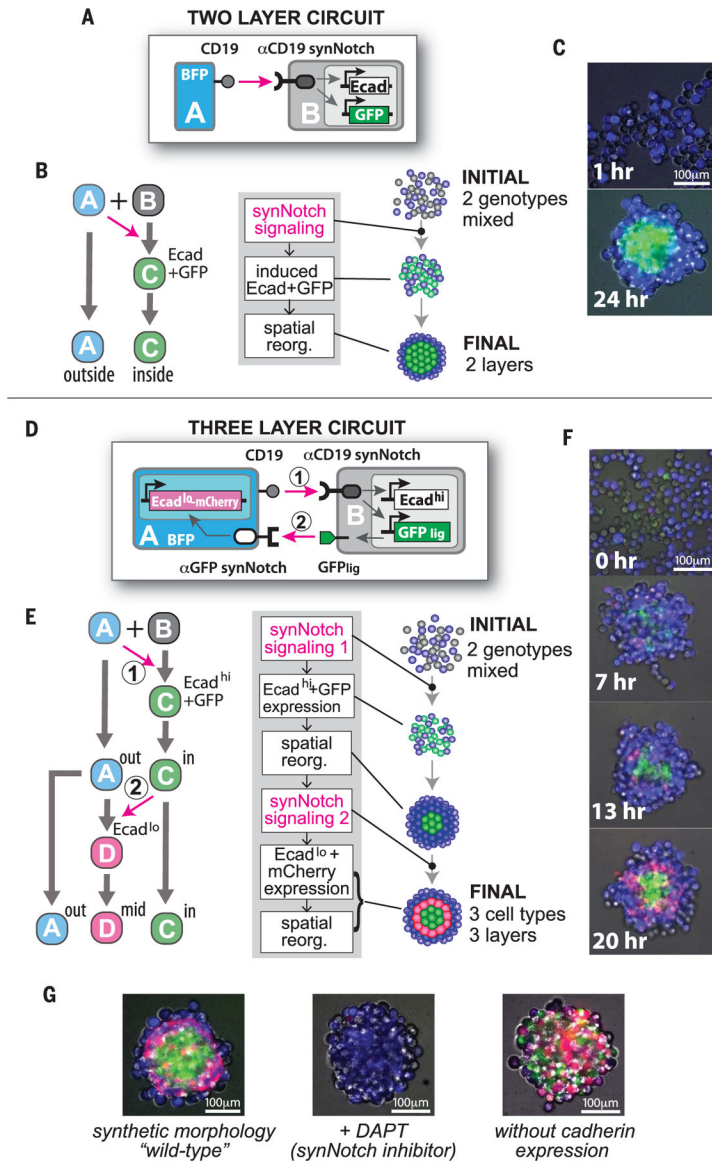
Fig. 2. Engineering self-organizing multilayered spheroids.
