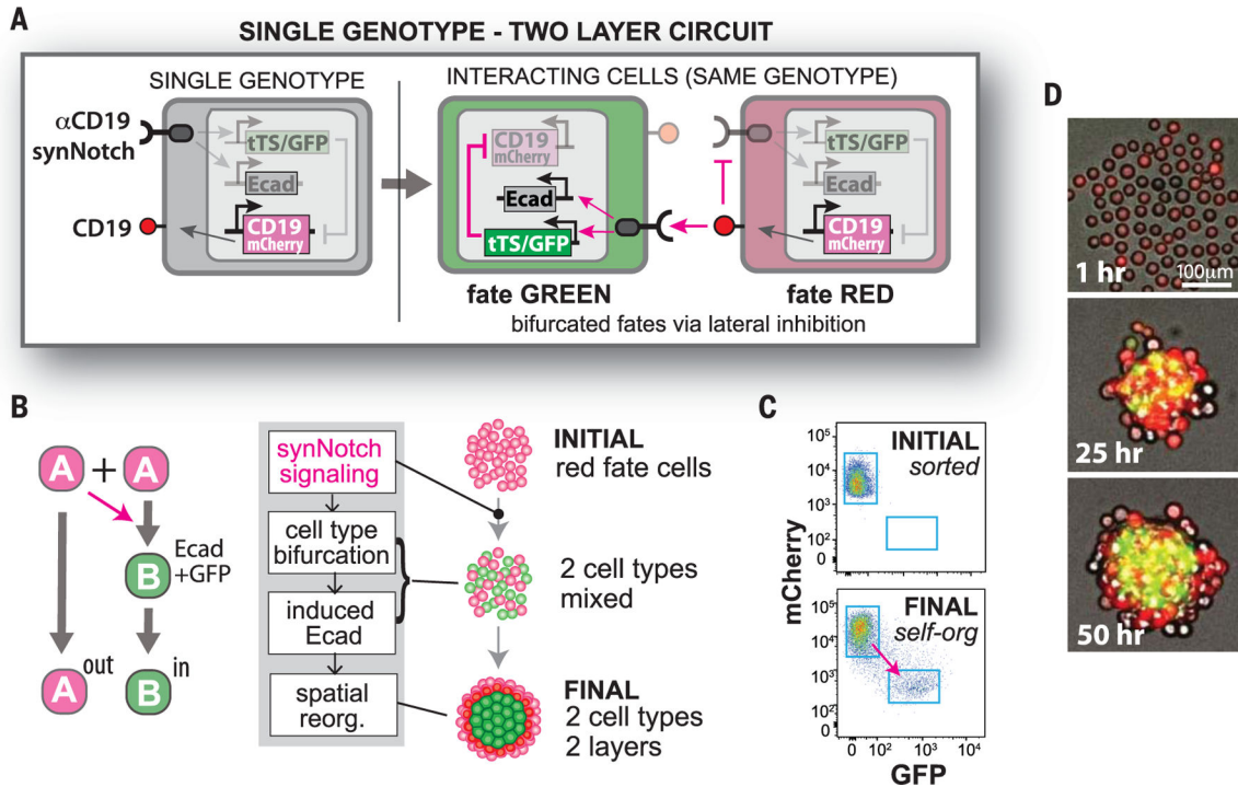
Fig. 4. Single-genotype circuit that induces fate bifurcation and spatial ordering into a two-layer structure.
