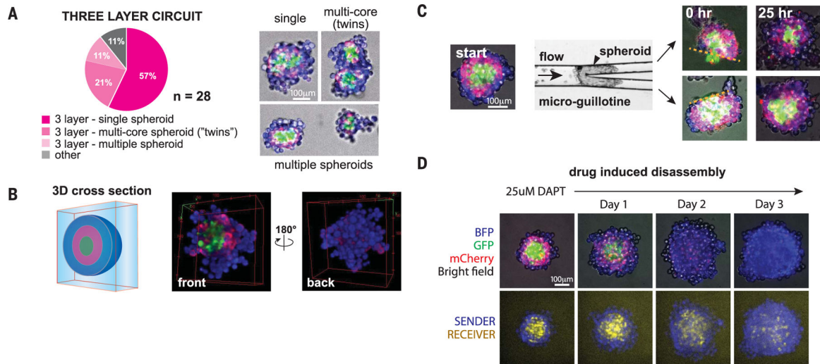
Fig. 3. Three-layer self-organized structure is robust, reversible, and self-repairing.
