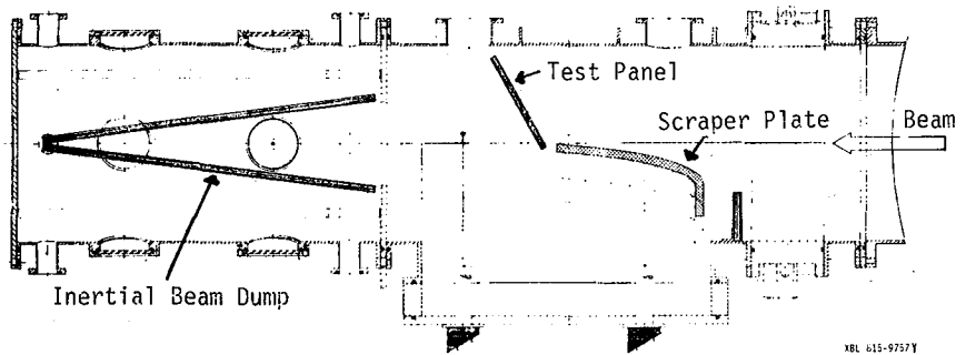
Figure 4: Prototype Panel Test
