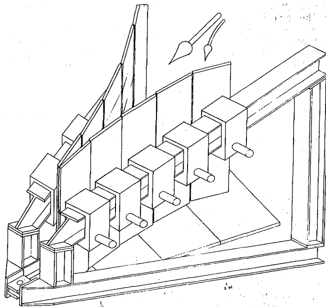
Figure 2: NBETF Ion Dump
