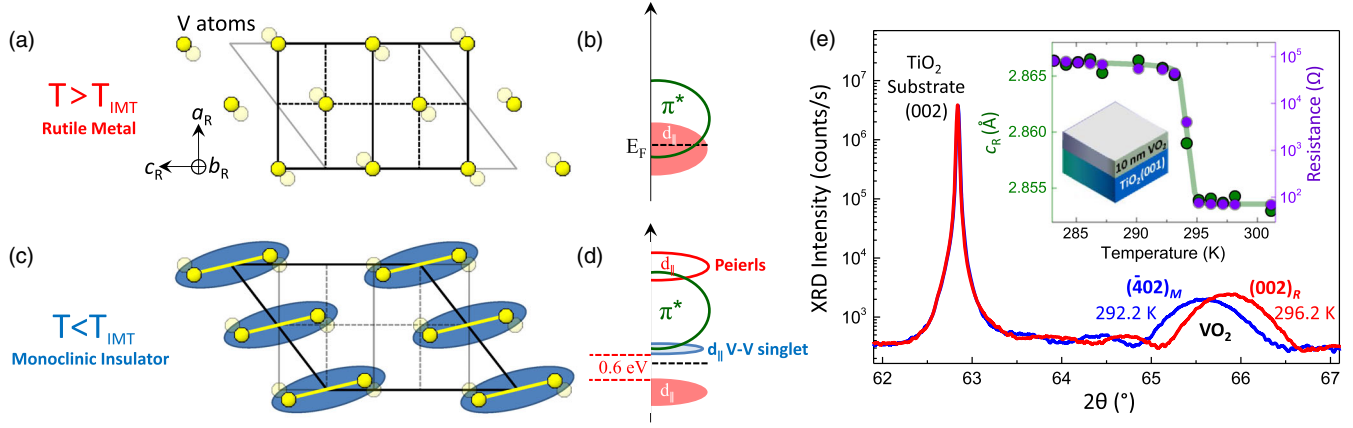
FIG. 1. (a) In the high-temperature ( T > T_{\text{IMT}} ) metallic phase, \text{VO}_2 forms rutile lattice structure with P4_2/mnm space symmetry where V atoms (yellow) occupy centers of sixfold oxygen-coordinated sites (O atoms not shown). (b) The near-Fermi-level t_{2g} states are separated in energy by the orthorhombic component of the crystal field into the twofold-degenerate e_g^\pi ( \pi^* ) states and a single a_{1g} orbital, which is aligned parallel to the rutile c axis ( c_R ) and is thus commonly denoted d_{\parallel} . The two bands overlap in energy, and the resulting nonzero density of states at the Fermi level accounts for the metallic behavior of the rutile phase [13,18]. (c) In the low-temperature ( T < T_{\text{IMT}} ) insulating phase the lattice undergoes a structural transition to a lower-symmetry ( P2_1/c ) monoclinic crystal system via dimerization of the neighboring V atoms along the c_R direction and tilting of the resultant V-V dimers along the rutile [110] and [\bar{1}\bar{1}0] directions. Each dimerized V-V atomic pair shares a singlet electronic state composed of two strongly correlated V 3d^1 electrons (shown in blue) [18]. (d) V-V dimerization splits the highly directional d_{\parallel} orbitals into the bonding and antibonding bands, and the tilting of the dimers shifts the \pi^* band to higher energies due to the increase of the p - d orbital overlap [13,18], together producing an insulating gap of 0.6 eV—the key aspect of the monoclinic phase observed via a wide variety of experimental techniques [23,24]. An additional d_{\parallel} feature in DOS, which arises at the onset of the conduction band (shown in blue), is a unique fingerprint of the strong electron-electron correlations within the dimers [18], accessible experimentally via polarization-dependent XAS at the O K edge (see Ref. [25] and this work). (e) Temperature-dependent x-ray diffraction \theta - 2\theta scans across the \text{TiO}_2 substrate (002) and the \text{VO}_2 film peaks show a clear structural transition in \text{VO}_2 manifested by an abrupt change in the interplanar atomic spacing along the direction normal to the film surface at 295 K (inset). Concomitant XRD and electronic transport measurements were collected for the heating cycle, with 1 h temperature equilibration time between scans. Inset: Temperature-dependent resistance (purple circles) and c_R lattice parameter (green circles) obtained concomitantly via electronic transport and x-ray-diffraction measurement, respectively. See full data set in the Supplemental Material [26].
