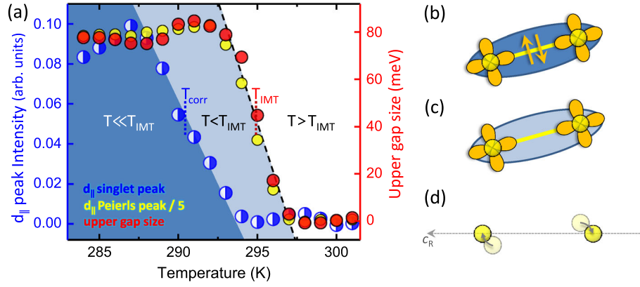
FIG. 3. (a) Temperature-dependent evolution of the d_{\parallel} V-V singlet peak intensity (blue and white symbols) showing distinctly different transition temperature ( T_{\text{corr}} = 290 K) as compared to the T_{\text{IMT}} (295 K), the critical temperature at which the collapse of the upper band gap (red solid symbols) as well as the structural transition (yellow solid symbols) is observed in \text{VO}_2 . Upper gap size is estimated by fitting the edge threshold with a polynomial function and extracting the energy (position along the x axis) of the half-maximum point from the fitted curve. Error bar analysis is presented in the Supplemental Material [26]. (b)–(d) Schematic representation of the three phases of \text{VO}_2 implied by the experimental data in the plots on the left. (b) The low-temperature phase ( T \ll T_{\text{IMT}} ) is a monoclinic insulator with a strongly correlated singlet electronic state on each V-V dimer. At T = T_{\text{corr}} the strong Coulomb correlations within the dimers soften, giving rise to a new monoclinic insulating phase shown in (c) via a purely electronic phase transition. Finally, only after the e - e correlations are sufficiently diminished ( T = T_{\text{corr}} + 3 K), the system undergoes a transition to a rutile metallic phase shown in (d).
