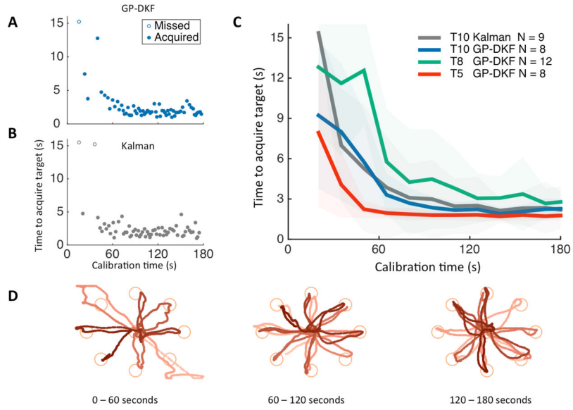
Fig. 2. Rapid calibration during the Radial-8 task. Participant T10 performed a three-minute calibration sequence with either the GP-DKF ( A ) or the Kalman ( B ) decoders. Targets were acquired when the cursor overlapped the target for 300ms, with a 15-second timeout. ( C ). Multiple calibration sequences from participants T5 (red), T8 (green) and T10 (blue) were done using the GP-DKF decoder, and with the Kalman decoder in T10 (grey). The thin dark lines are the average amount of time to acquire a target across all blocks (shaded area is \pm 1 standard deviation). Averages are computed by binning data in 15-second increments, with a 5 second offset from calibration start. ( D ). Example cursor trajectories during calibration using the GP-DKF decoder (participant T5). The brightness goes from light to dark as time elapses during the 60 second interval of closed-loop neural cursor control. Data were used from trial days: 30 and 33 (T5); 662, 665, (T8); and 112, 203, 215, 236 (T10).
