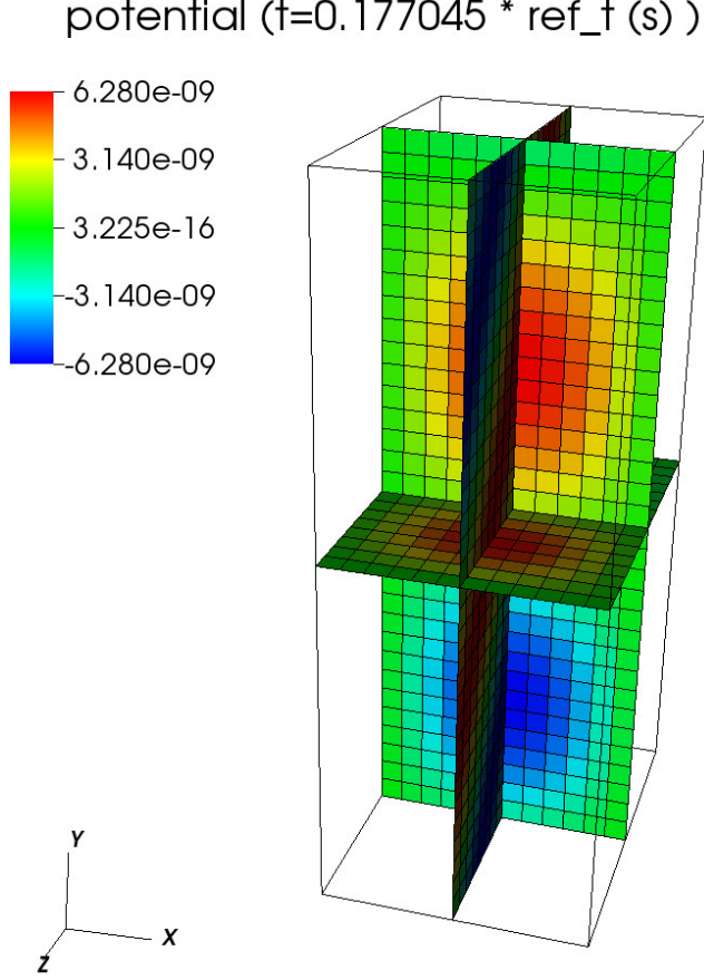
Figure 4.5: 3D electrostatic potential distribution normalized to \phi_0 = 400\text{V} . The normalization number (ref.t) for the time variable is 5.11 \times 10^{-6} s.
