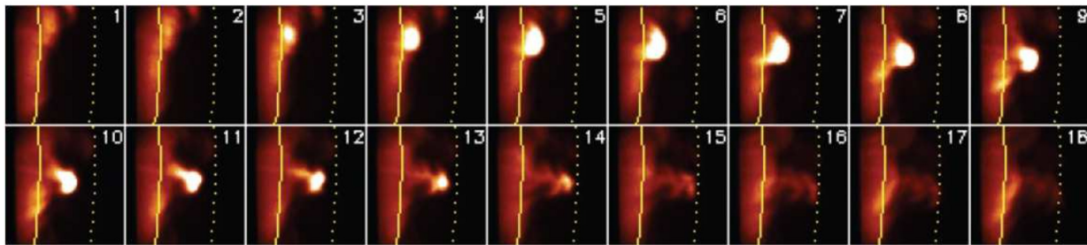
Figure 1.2: Blob creation and propagation in the SOL of the NSTX tokamak [24]. The images are produced from GPI diagnostics. The radius of the blob is approximately \sim 2 cm, and the propagation speed is in the order of \sim 1 km/s.
