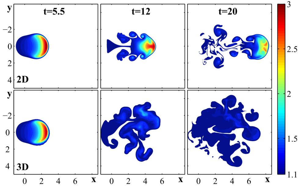
Figure 1.3: Comparison of density contours from 2D (top) and 3D (bottom) simulation [28]. The 3D simulation exhibits significant dissipation of the blob structure due to RDWI.
