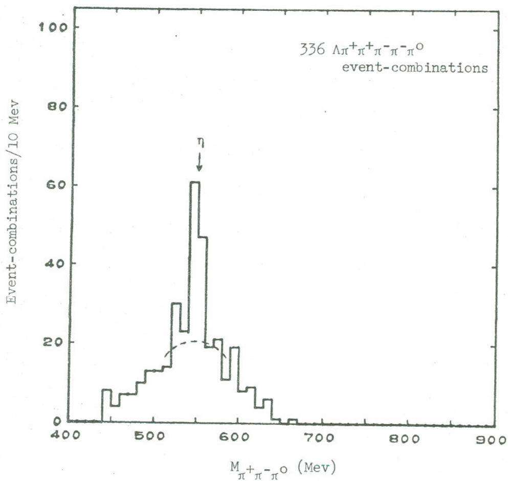
Figure 6. The projection of Figure 5 onto the M_{\pi^+\pi^-\pi^0} axis for those \Lambda\pi^+\pi^+\pi^-\pi^-\pi^0 events with 950 \leq M_{\pi^+\pi^+\pi^-\pi^-\pi^0} \leq 970 Mev. Again each event appears four times. The peak at the \eta mass, measured from the dashed line upward, contains one-quarter of the event-combinations.
