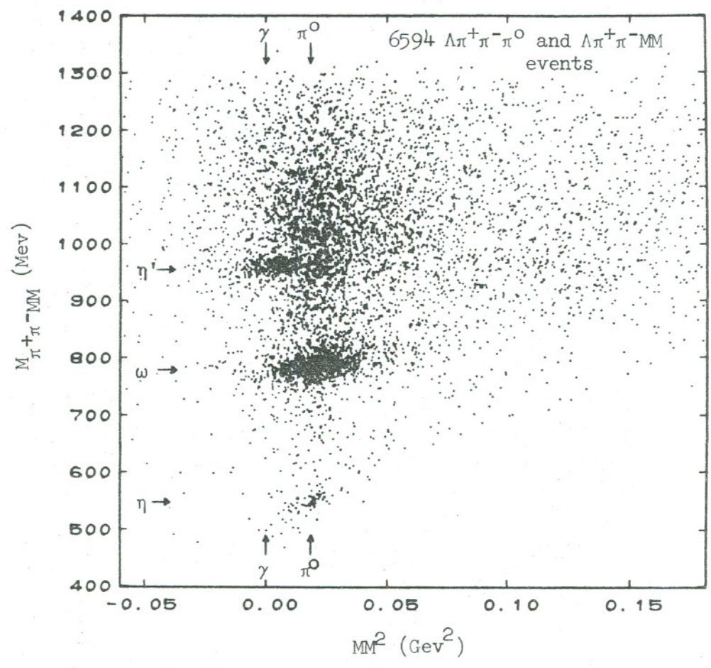
Figure 16. Plot of M_{\pi^+\pi^-\text{MM}} versus MM^2 for low \Delta^2 events fitting either \Lambda\pi^+\pi^-\pi^0 or \Lambda\pi^+\pi^-\text{MM} , but having no acceptable fit for \Lambda\pi^+\pi^- or \Sigma^0\pi^+\pi^- . For the \Lambda\pi^+\pi^-\pi^0 events, MM represents the unfitted mass recoiling against the \Lambda\pi^+\pi^- system. The arrows labeled \gamma and \pi^0 indicate the centers of the two vertical bands where \Lambda\pi^+\pi^-\gamma and \Lambda\pi^+\pi^-\pi^0 events should appear, respectively.
