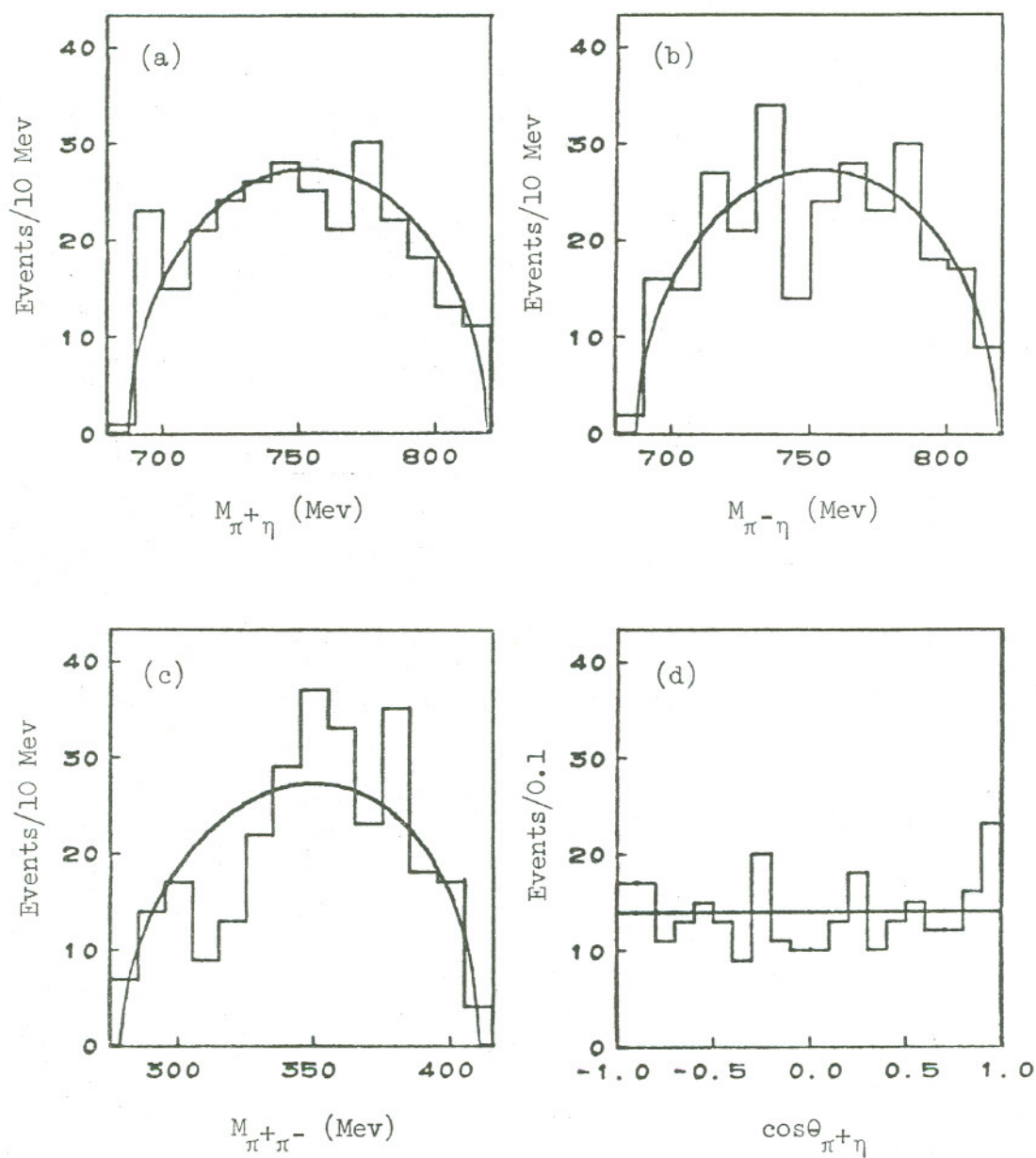
Figure 27. Four projections of the Dalitz plot for the 278 \pi^+\pi^-\eta_N events of Figure 26. The projections are (a) M_{\pi^+\eta} , (b) M_{\pi^-\eta} , (c) M_{\pi^+\pi^-} , and (d) \cos\theta_{\pi^+\eta} . The angle \theta_{\pi^+\eta} is measured in the dipion rest frame. The curves represent phase space.
