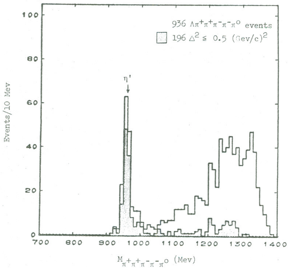
Figure 3. The M_{\pi^+\pi^+\pi^-\pi^-\pi^0} mass spectrum for events fitting the reaction K^-p \rightarrow \Lambda\pi^+\pi^+\pi^-\pi^-\pi^0 . The shaded events are those with \Delta^2 \leq 0.5 \text{ (Gev/c)}^2 .
