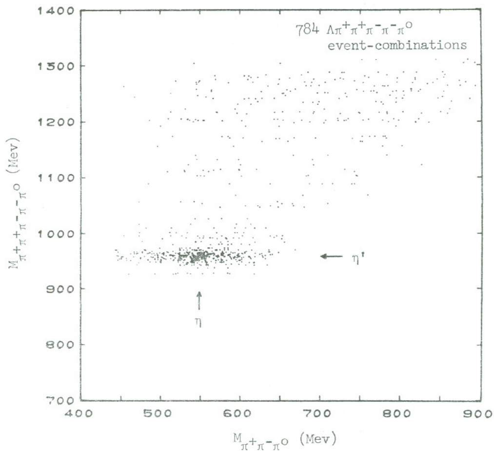
Figure 5. M_{\pi^+\pi^+\pi^-\pi^-\pi^0} versus M_{\pi^+\pi^-\pi^0} for \Lambda\pi^+\pi^+\pi^-\pi^-\pi^0 events with low \Delta^2 . Each event is plotted four times, representing the four \pi^+\pi^-\pi^0 combinations which can be formed.
