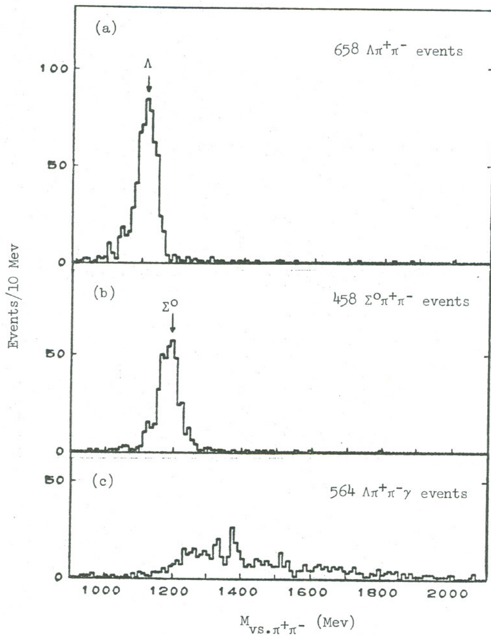
Figure 21. Plots of the unfitted mass M_{vs.\pi^+\pi^-} recoiling against the \pi^+\pi^- system in the reprocessed events assigned to the hypotheses: (a) \Lambda\pi^+\pi^- ; (b) \Sigma^0\pi^+\pi^- ; and (c) \Lambda\pi^+\pi^-\gamma .
