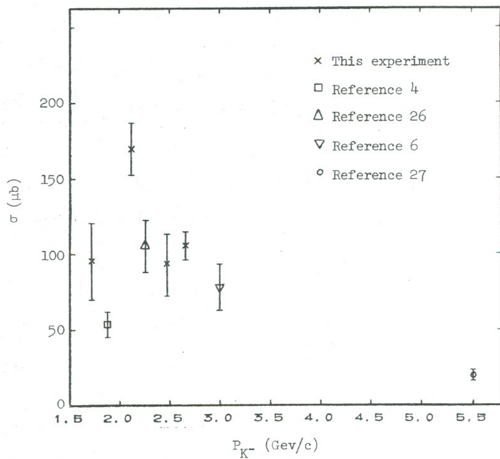
Figure 43. Plot of the total cross section for production of \eta' in the reaction K^-p \rightarrow \Lambda\eta' , as a function of the beam momentum, P_{K^-} .
