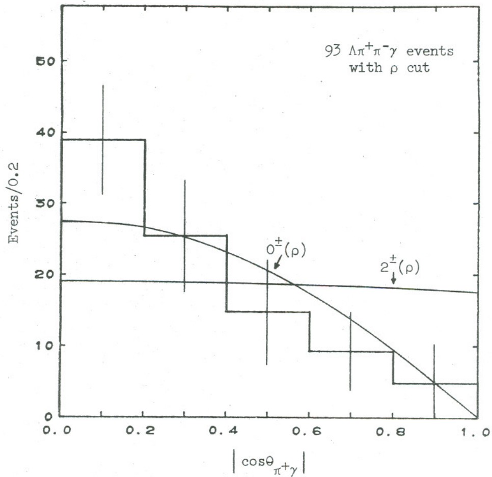
Figure 41. The folded \cos\theta_{\pi^+\gamma} distribution for low \Delta^2 \pi^+\pi^-\gamma events having 945 \leq M_{\pi^+\pi^-\gamma} \leq 975 Mev and a cut of 640 \leq M_{\pi^+\pi^-} \leq 800 Mev to favor \rho events. A background subtraction has been carried out. The curves indicate the predictions for C = +1 , J^P = 0^+ and 2^+ , with \rho assumed.
