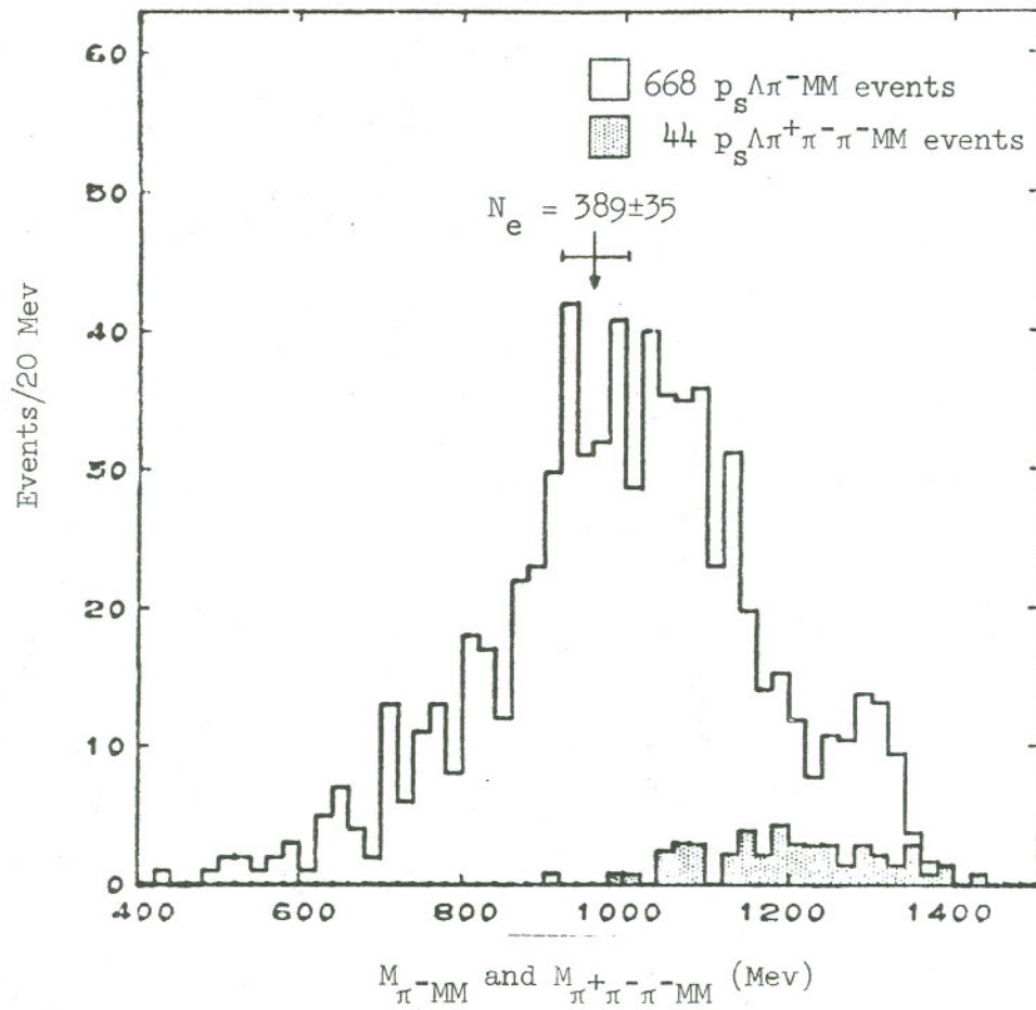
Figure 51. Plot of the \pi^-MM and \pi^+\pi^-\pi^-MM (shaded) mass spectra from K^-d \rightarrow p_s \Lambda \pi^-MM and K^-d \rightarrow p_s \Lambda \pi^+\pi^-\pi^-MM events, respectively. Only events having \Delta_{n-\Lambda}^2 \leq 0.7 (Gev/c) ^2 have been plotted. The arrow and cross-bar indicate where the N_e expected \eta' events would appear if I_{\eta'} were 1.
