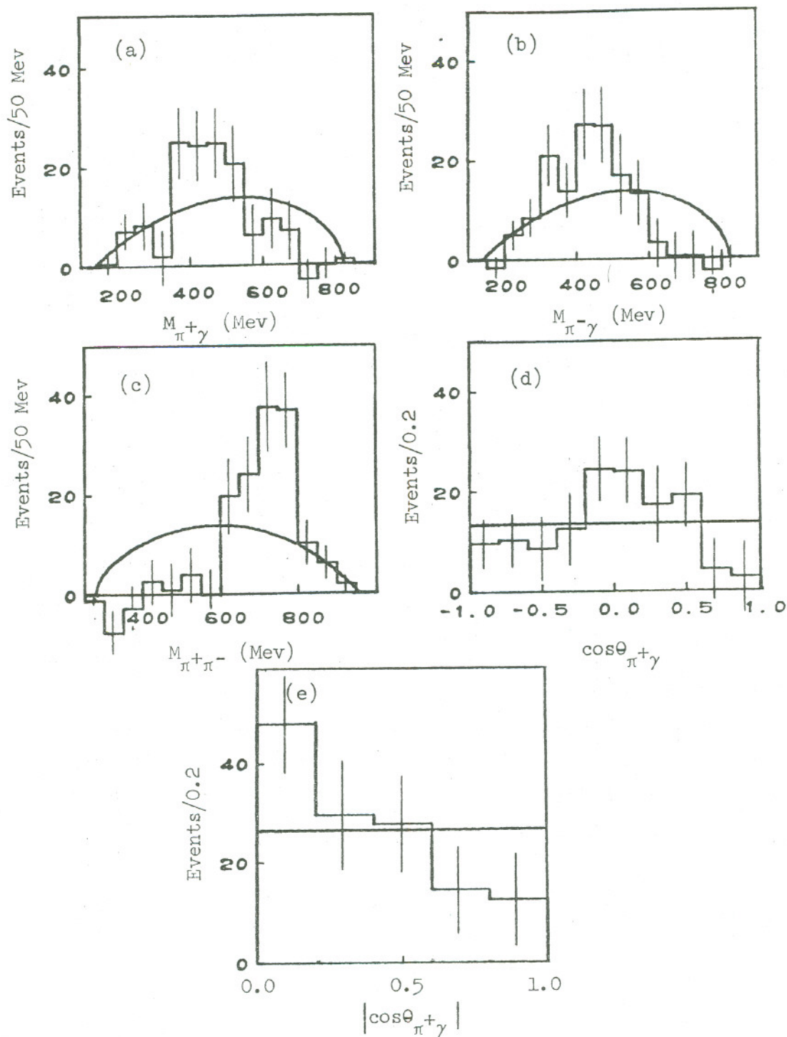
Figure 39. The Dalitz plot projections for the 132 low \Delta^2 \pi^+\pi^-\gamma events, having 945 \leq M_{\pi^+\pi^-\gamma} \leq 975 Mev, which remain after the subtraction discussed in the text has been carried out. The projections are (a) M_{\pi^+\gamma} , (b) M_{\pi^-\gamma} , (c) M_{\pi^+\pi^-} , (d) \cos\theta_{\pi^+\gamma} , and (e) |\cos\theta_{\pi^+\gamma}| . The curves again represent phase space.
