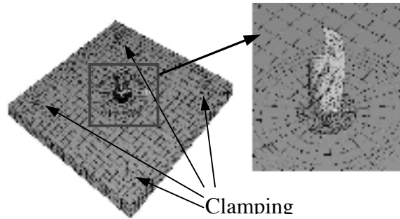
Figure 1. A finite element meshes of a two-layered workpiece and a drill.
