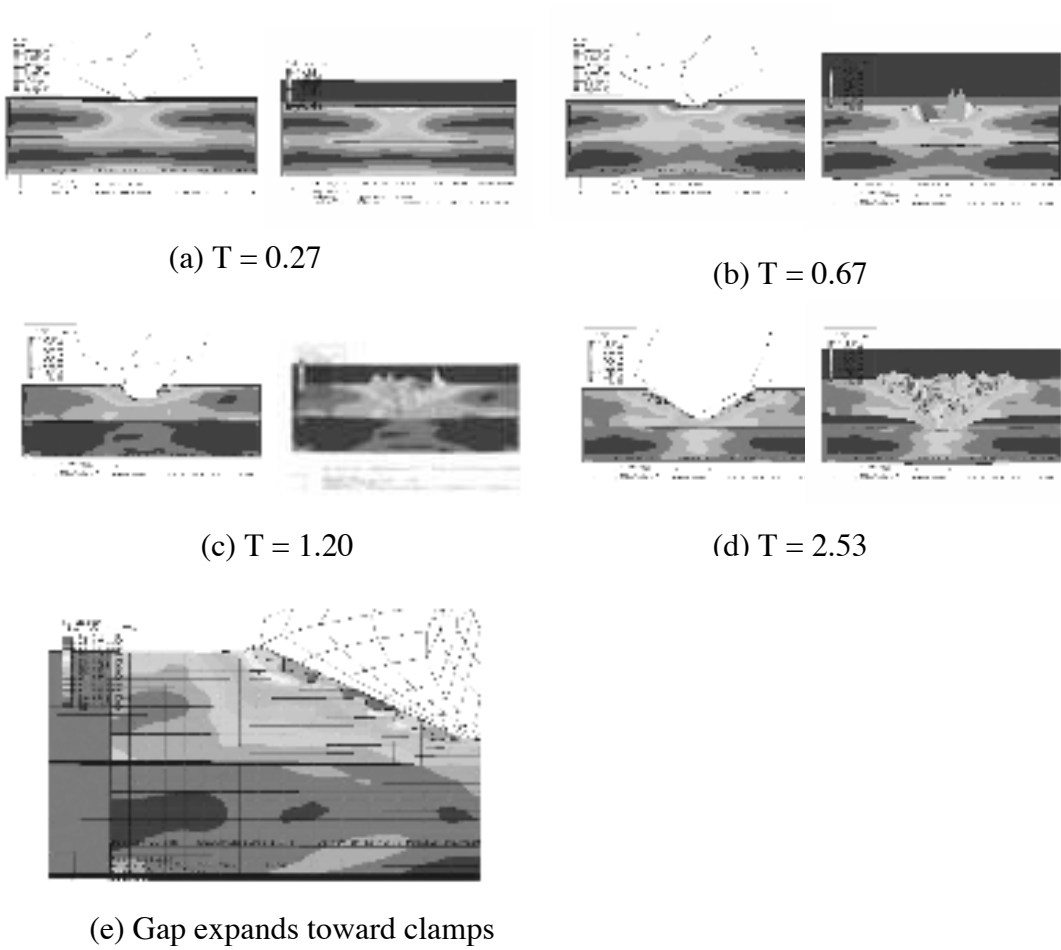
Figure 2. FE simulation of gap formation process.
