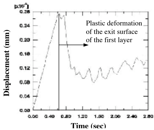
Figure 3. Displacement of the edge of the hole.
