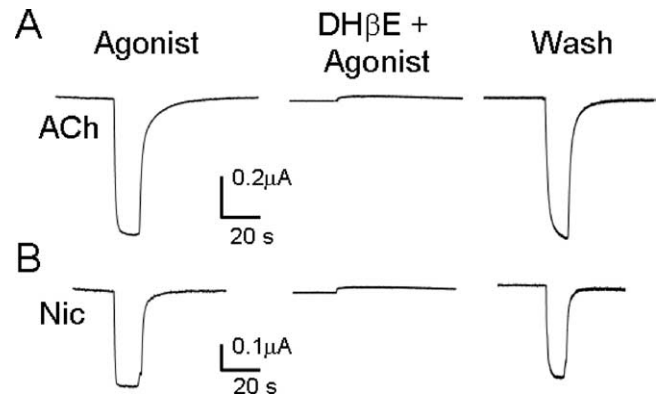
Figure 5. Reversible block of ( \alpha 4\text{L9}'\text{A} ) \beta 2 receptors expressed in oocytes by 0.2 \mu M DH \beta E. A , B , Agonist concentration in each case was the \text{EC}_{20} for ACh (0.125 \mu\text{M} , A ) or Nic (0.025 \mu\text{M} , B ), applied for 15 s. Left, first agonist application. Oocytes were washed with recording buffer for 2 min (not shown) and then perfused with 0.2 \mu M DH \beta E for 5 min. Middle, The subsequent response to coapplied agonist + 0.2 \mu M DH \beta E. Oocytes were then washed with buffer for 5 min, and an additional 15 s application of agonist was given (right). These data are typical of n > 5 oocytes for each agonist. The small outward deflections are solution change artifacts.
