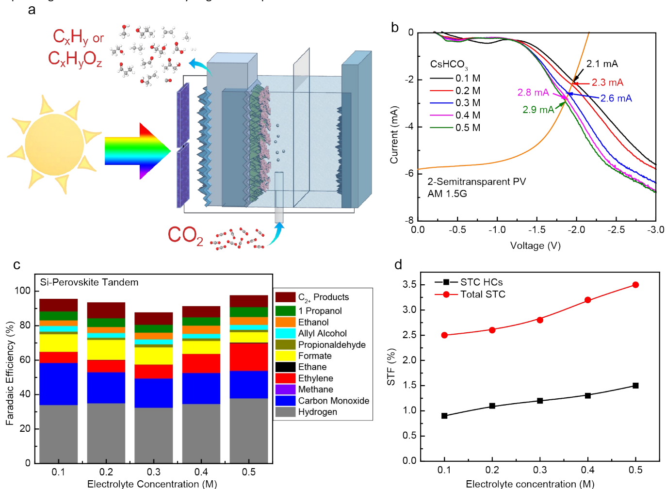
Figure 5. Solar-driven \text{CO}_2\text{R} measurements performed in a two-electrode configuration with a Si photocathode and an \text{IrO}_2 nanotube anode in tandem with two series-connected semi-transparent perovskite solar cells. a , Schematic of solar \text{CO}_2 reduction PV-PEC system. b , Measured current of top photoabsorbers (perovskite solar cells) and bottom photoabsorber (Si photocathode) in various electrolyte conditions (0.1 – 0.5 M \text{CsHCO}_3 ) and under 1-sun illumination. Light reaching the Si photocathode is filtered via the top absorber; PEC measurements were performed in 2-electrode configuration. Intersection of these current shows the operating point of the device. c , \text{CO}_2\text{R} product distribution of PV-PEC tandem device in 0.1 to 0.5 M \text{CsHCO}_3 and under 1-sun illumination. d , Solar-to-chemical conversion efficiency of PV-PEC device as a function of electrolyte concentration.
