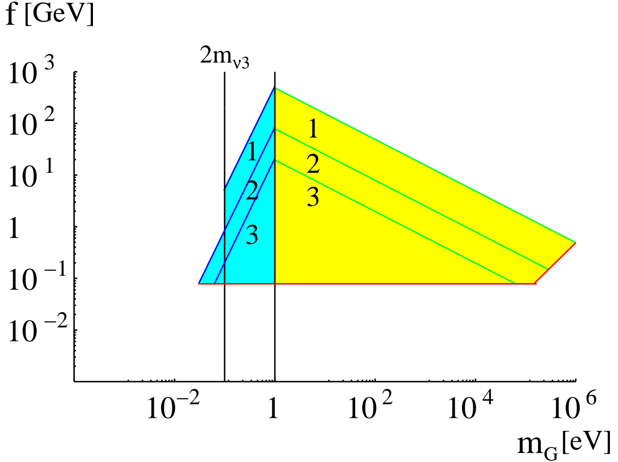
FIG. 3: The signal regions and bounds for three Majorana neutrinos with hierarchical masses m_\nu = 0.05, 0.008, 0.002 eV. The regions are labeled by the number of neutrinos species that recouple to the pseudo-Goldstone boson for m_G > 1 eV and by the number of neutrinos that scatter at T \sim 1 eV for m_G < 1 eV.
