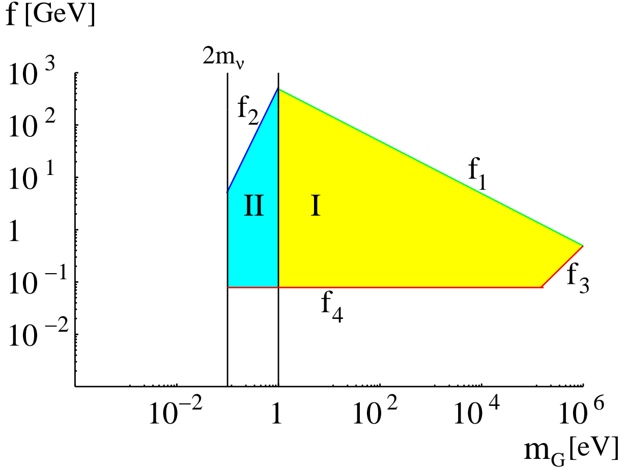
FIG. 1: Signal regions and cosmological bounds for a single Majorana neutrino coupled to a single pseudo-Goldstone boson. The lines and regions are labeled as in the text. CMB signals occur throughout the two shaded regions. The area below f_3 and f_4 is excluded by BBN, and in the region above f_1 and f_2 the PGB is too weakly coupled to give any signal. There is an energy density signal in region I and a scattering signal in region II. We have assumed m_\nu = 0.05 eV \lambda = 1 .
