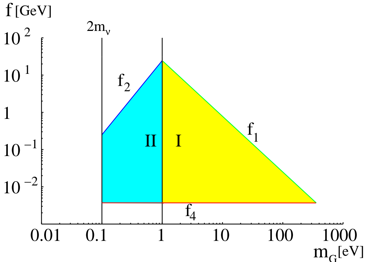
FIG. 2: Signal regions and cosmological bounds for a single Dirac neutrino coupled to a single pseudo-Goldstone boson. The region below line f_4 is excluded by BBN. In the region above lines f_1 and f_2 the Goldstone boson is too weakly coupled to give any signal. There is a signal in \rho_{rel} in region I, and in region II there is an overall phase shift. We have assumed m_\nu = 0.05 eV, \lambda = 1 and r = 0.0001 . The lower bound on f scales as f_4 \propto r^{1/3} .
