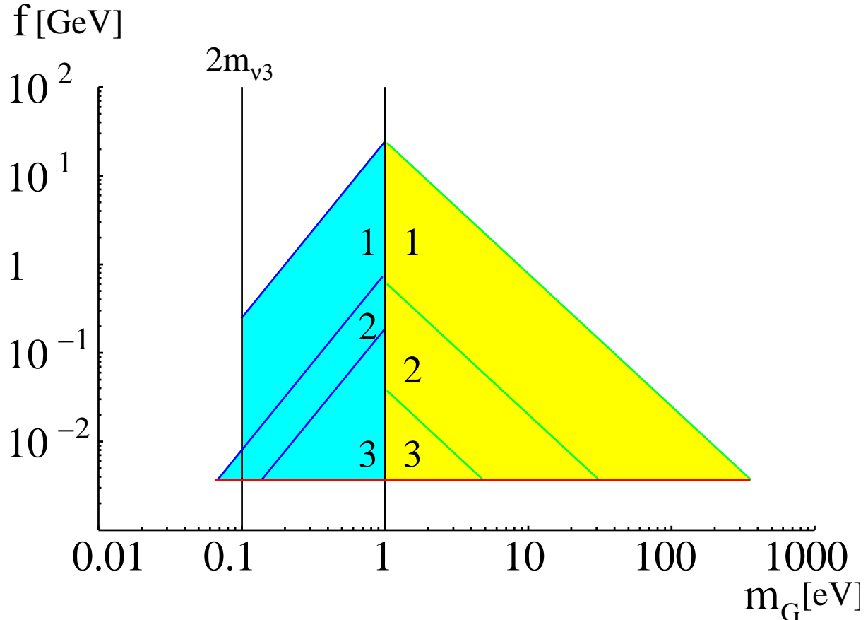
FIG. 4: The signal regions and bounds for three Dirac neutrinos with hierarchical masses m_\nu = 0.05, 0.008, 0.002 eV. The regions are labeled by the number of neutrinos species that recouple to the pseudo-Goldstone boson for m_G > 1 eV and by the number of neutrinos that scatter at T \sim 1 eV for m_G < 1 eV and r = 0.0001 .
