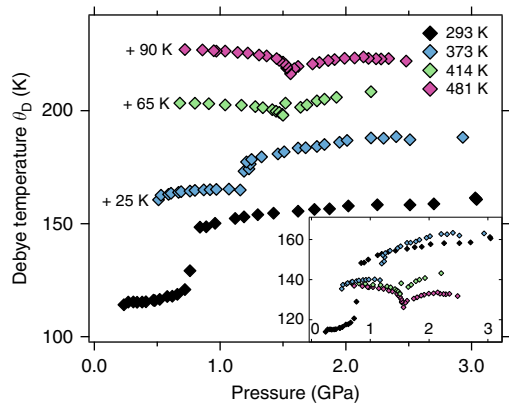
Fig. 6 Debye temperatures of polycrystalline cerium. They are shown versus pressure (uncertainty < 0.05 GPa) at different temperatures. Symbols are larger than the experimental uncertainties
