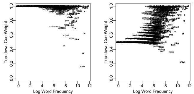
Figure 2: Frequent words have the chance to depart from their initial weights, whether those weights are at maximum (left) or in the middle of the range (right).
