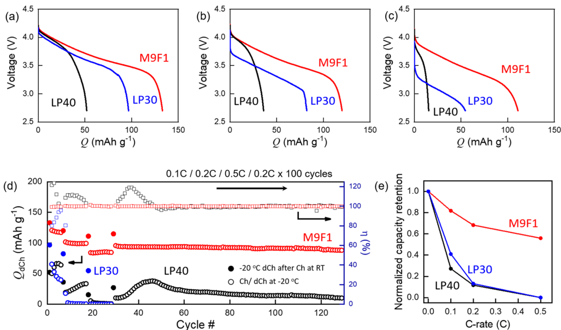
Figure 3. Low-temperature electrochemical performance of NMC111||graphite type pouch cells using different electrolytes. Voltage profiles during discharge at (a) 0.1C, (b) 0.2C, and (c) 0.5C under -20\text{ }^{\circ}\text{C} after room-temperature charge at 0.1C. (d) Charge and discharge cycling performance of cells at different C-rates (0.1C, 0.2C, and 0.5C) using different electrolytes. The cycling test was conducted on 0.1C for 5 cycles, 0.2C for 10 cycles, 0.5C for 10 cycles, and 0.2C for 100 cycles. The first closed circle at each C-rate is the first discharge capacity after charge at room-temperature. Following open circles are the repeated charge and discharge cycling after discharge at the same rate at -20\text{ }^{\circ}\text{C} . (e) The normalized capacity retention at first charge from panel d.
