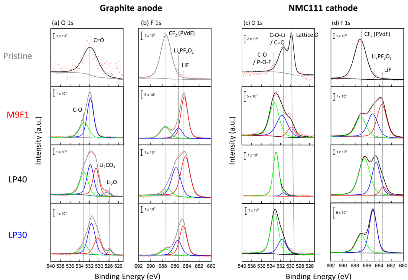
Figure 5. Characterization of electrode surfaces by XPS. (a) O 1s and (b) F 1s regions for graphite anodes; (c) O 1s and (d) F 1s regions for NMC111 cathodes. All the electrodes were obtained from cells after the cycling test described in Figure 3d.
