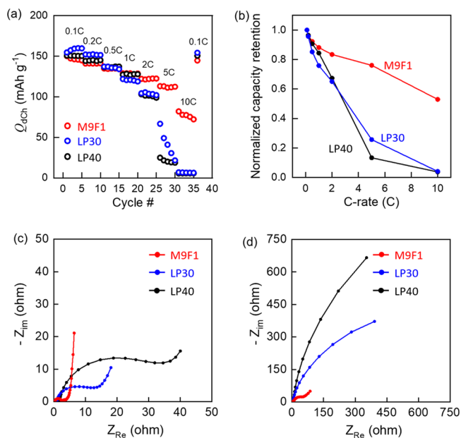
Figure 2. Rate performance results of the NMC111||graphite pouch cells and EIS analysis data of the cell at 0% SOC after cycling. (a) Rate capabilities of full cells evaluated between 2.7 and 4.3 V voltage window using different electrolytes. All the cells have the same cathode and anode configuration, and the cell capacity was calculated and referred to the cathode mass. (b) The normalized capacity retention from the discharge capacity of 0.1C. Nyquist plots of the cells after rate capabilities at the different temperature between (c) room-temperature (RT) and (d) -20\text{ }^{\circ}\text{C} .
