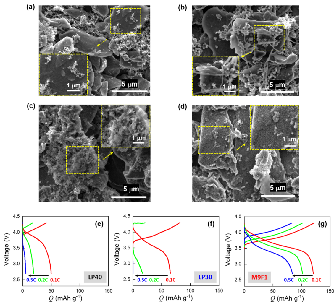
Figure 6. SEM images of the pristine and cycled graphite electrodes at -20\text{ }^{\circ}\text{C} . All the cycled electrodes were obtained from cells after cycling test described in Figure 3d: (a) pristine graphite and graphite cycled in LP40 (b), LP30 (c), and M9F1 (d). Potential profiles at the first charge and discharge cycle of cells with (e) LP40, (f) LP30, and (g) M9F1 electrolyte at -20\text{ }^{\circ}\text{C} .
