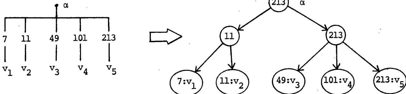
Figure 4c—Dataflow structure represented as a 2-3 tree
