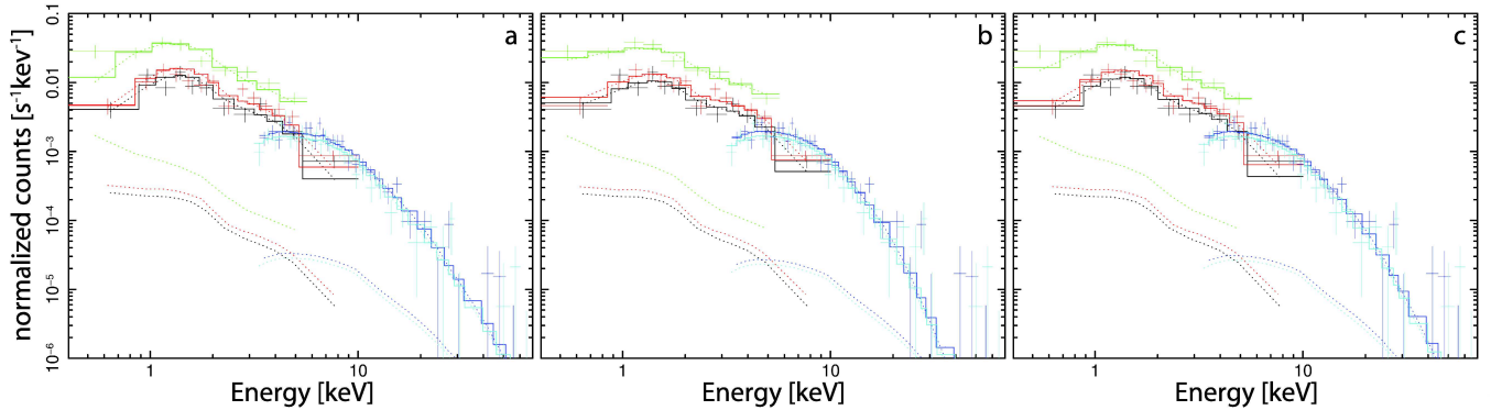
FIG. 7.— Panel (a): Best-fit Mekal (zvphabs*mekal) to the combined NuSTAR+XMM observation. The model consists of two components: The lower dotted lines represent the fixed power-law model of the faint nearby sources (see text), and the upper dotted lines represent the zvphabs*mekal best-fit model to the SN 2010jl X-ray spectrum. The solid lines (stairs) show the best combined fit for each instrument, while the plus signs show the data with error bars. The instruments are NuSTAR FPM A (blue), NuSTAR FPM B (cyan), XMM PN (green), XMM MOS1 (black), and XMM MOS2 (red). The fit parameters are listed in Table 6. Panel (b): Like panel (a) but for zvphabs*powerlaw*spexpcut. Panel (c): Like panel (a) but for zvphabs*powerlaw*spexpcut with fixed \Gamma = 1 .
