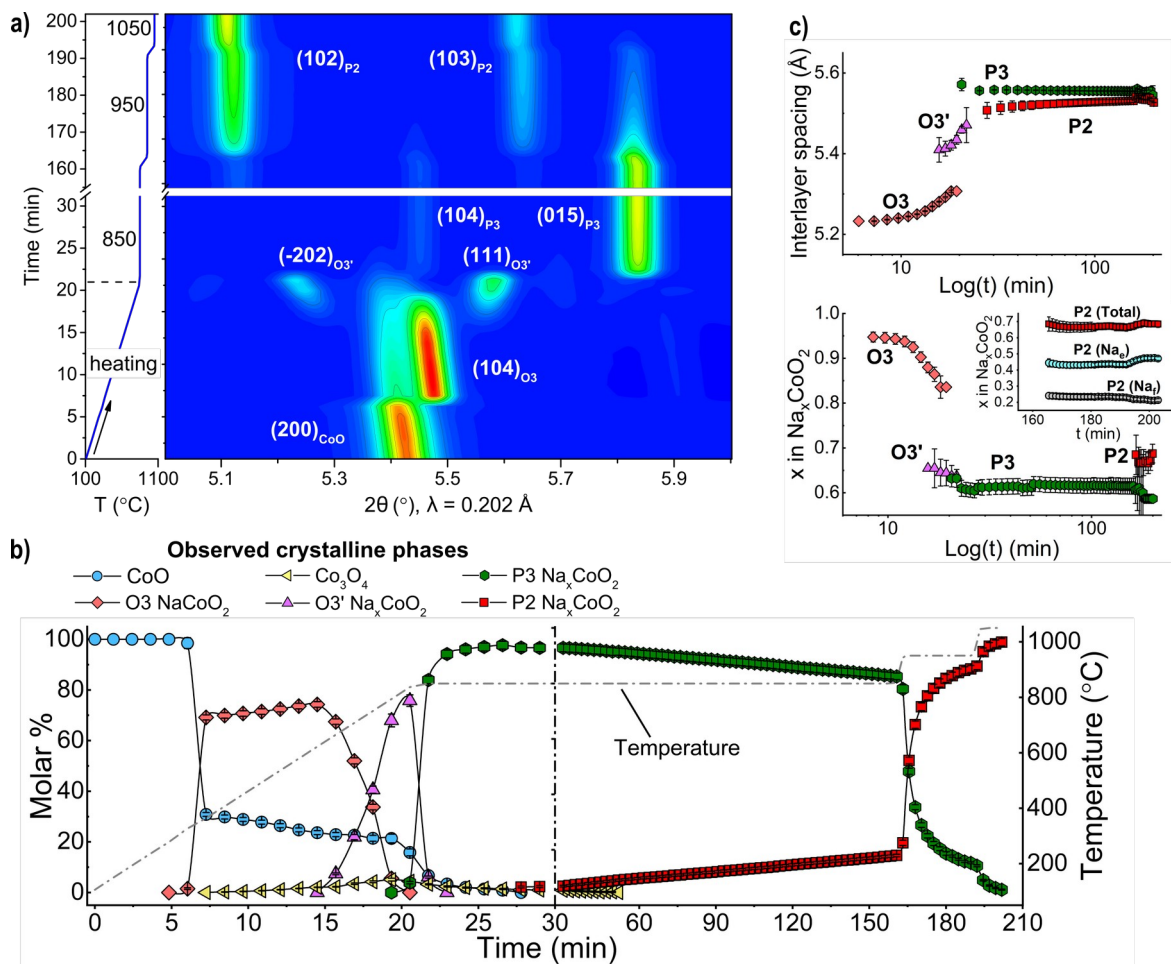
Figure 2: a) Solid-state synthesis of P2 Na_{0.7}CoO_2 monitored by in situ synchrotron XRD. The contour plot highlights the evolution of the Bragg peaks. A sequence of layered compounds is observed ( O3 \rightarrow O3' \rightarrow P3 \rightarrow P2 ). b) and c) Parameters obtained from Rietveld refinement of the XRD patterns. b) Evolution of the molar % of the observed crystalline phases and c) interlayer spacing and Na content of each Na_x CoO_2 polytype.
