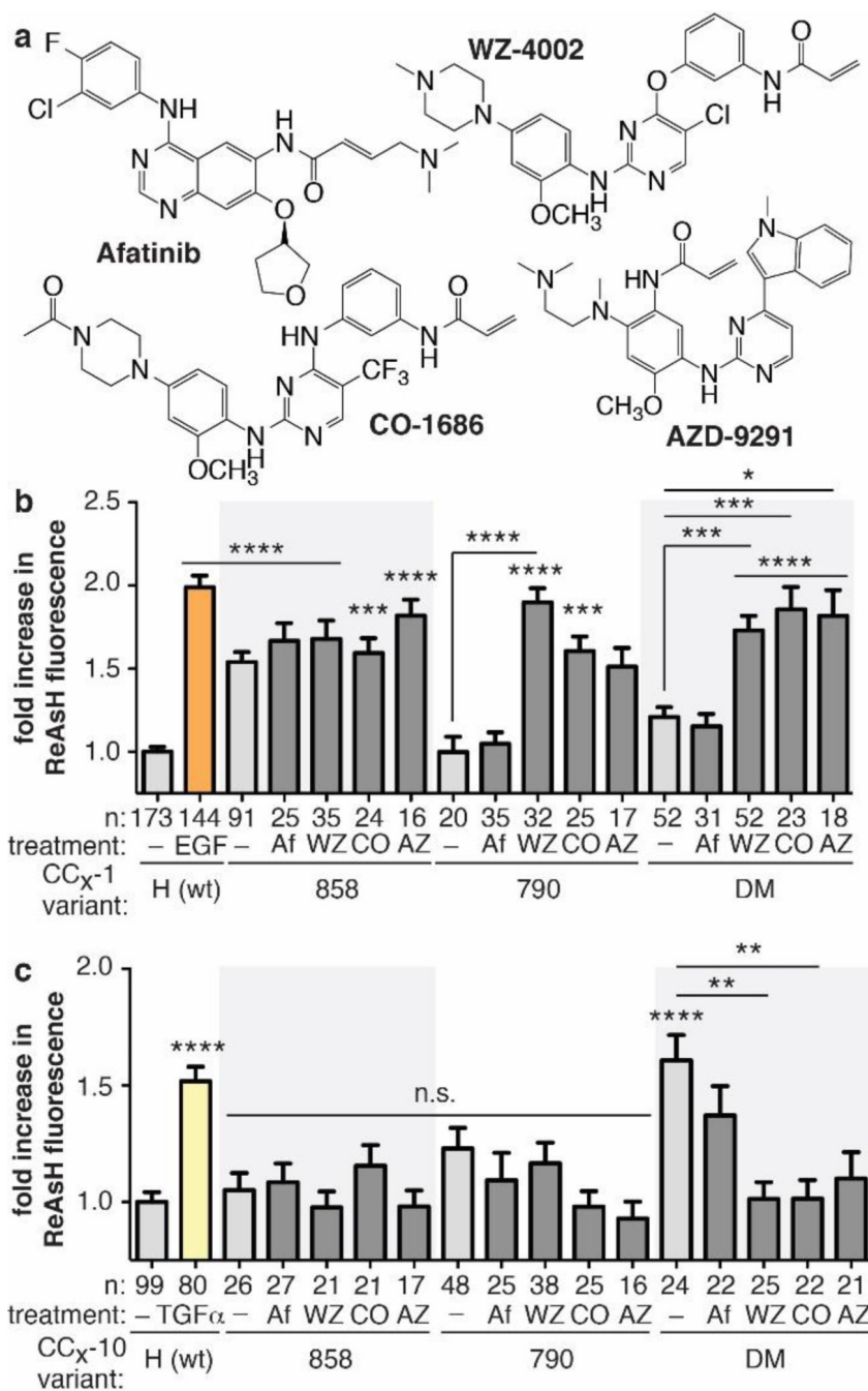
Figure 3. (A) Structures of afatinib (Af) 6 , WZ4002 (WZ) 5 , CO-1686 (CO) 7 , and AZD-9291 (AZ) 8 . (B,C) Fold-increase in expression-corrected ReAsH fluorescence over background of cells expressing CC x -1 or CC x -10 variants in the presence or absence of TKI. Error bars, s.e.m. **** p < 0.0001, *** p < 0.001, ** p < 0.01, * p < 0.05 from one way ANOVA with Bonferroni post-test.
