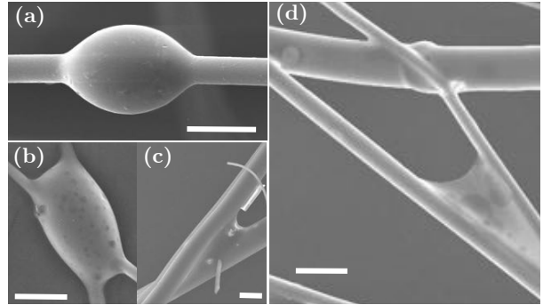
Figure 1: SEM pictures of drops of binder lying on glass wool. (a) Drop on a single fiber, (b) liquid in the drop state between two crossed fibers, (c) and (d) liquid in the column state between two fibers. Scale bars are 10\ \mu\text{m} (Pictures from Saint-Gobain Research, reproduced with permission from Bintein [21]).
