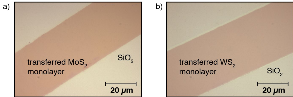
Figure S13. High-magnification white light optical images of a) \text{MoS}_2 and b) \text{WS}_2 monolayers on 260 nm \text{SiO}_2 substrates, produced using the transfer method described in this paper.
