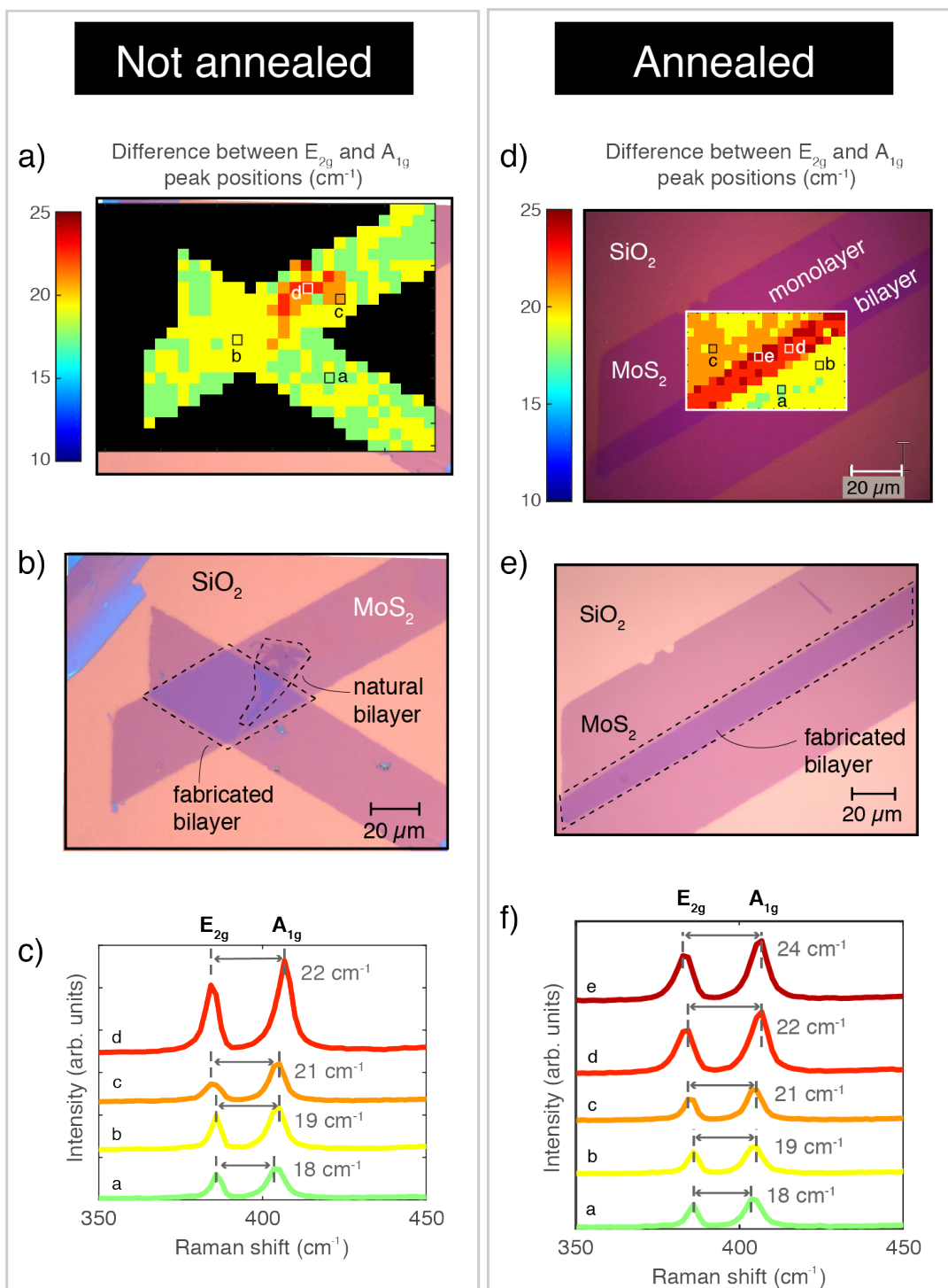
Figure S12. (a) Raman map of two crossed \text{MoS}_2 monolayer features, whose overlap forms a fabricated \text{MoS}_2 bilayer. The inter-peak difference is consistent with monolayer \text{MoS}_2 , except in the region where a natural bilayer is present, highlighted in (b). (c) Spectra from several points on the Raman map, indicating both monolayer and bilayer material are present. (d) Raman map of two overlapped \text{MoS}_2 monolayers, creating a fabricated bilayer, after a brief annealing step. The overlapping region now behaves as an \text{MoS}_2 bilayer, as indicated by the increased E_{2g} - A_{1g} peak difference (in \text{cm}^{-1} ). (e) The region mapped in (d). (f) Spectra from identified points of the region mapped in (d).
