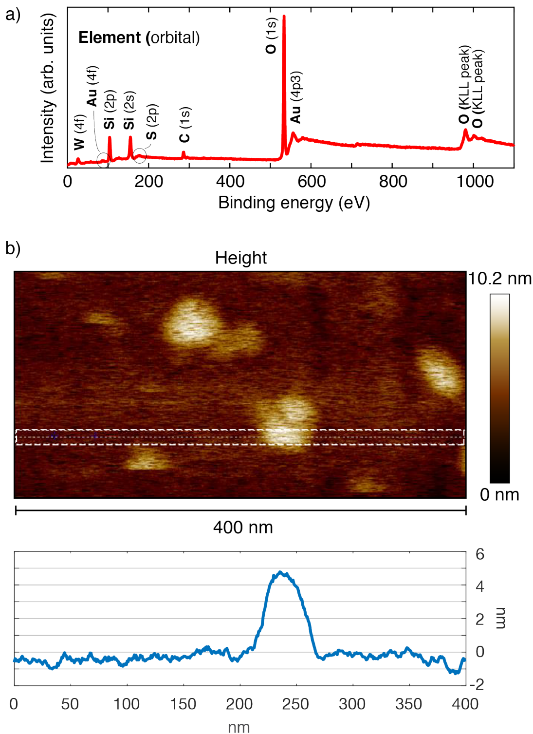
Figure S11. (a) XPS characterization of residual particles on \text{WS}_2 , indicating the presence of expected substrate elements (Si, O), TMDC elements (W, S), and calibration elements (C). The remaining identified element is Au, which may comprise the residual particles. (b) AFM topography map of the particles. The height of the region in the white dashed box is plotted in the accompanying line-scan, showing that the particles are \sim 50 nm wide and \sim 5 nm tall.
