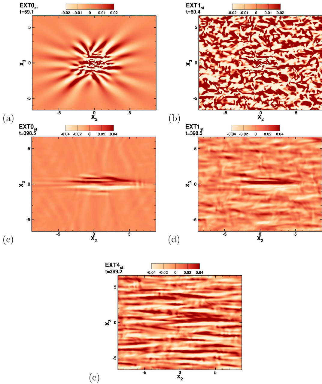
Figure 3.4: Comparison of the instantaneous \omega_1 at a x_2-x_3 plane for the stratified cases at t \approx 60 (a, b) and at t \approx 400 (c, d) between the undisturbed background and 1% external turbulence cases. The bottom snapshot corresponds to 4% external turbulence.
