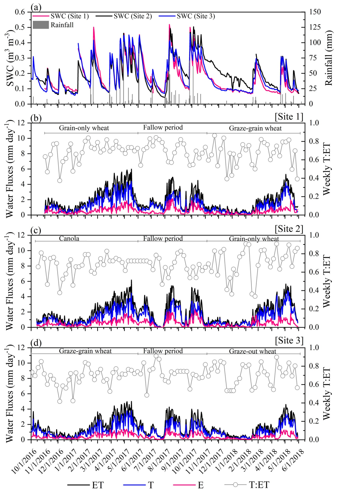
Figure 1. (a) Daily variations of rainfall and soil water content at each site, (b–d) daily variations of total evapotranspiration (ET), transpiration ( T ), and direct evaporation ( E ) based on flux variance similarity method at three different sites. Open circles plotted on the secondary Y -axis show the ratio of weekly T and ET. Notably, all three sites underwent crop rotation. Fallow period and canola were not considered for analyses in this study.
