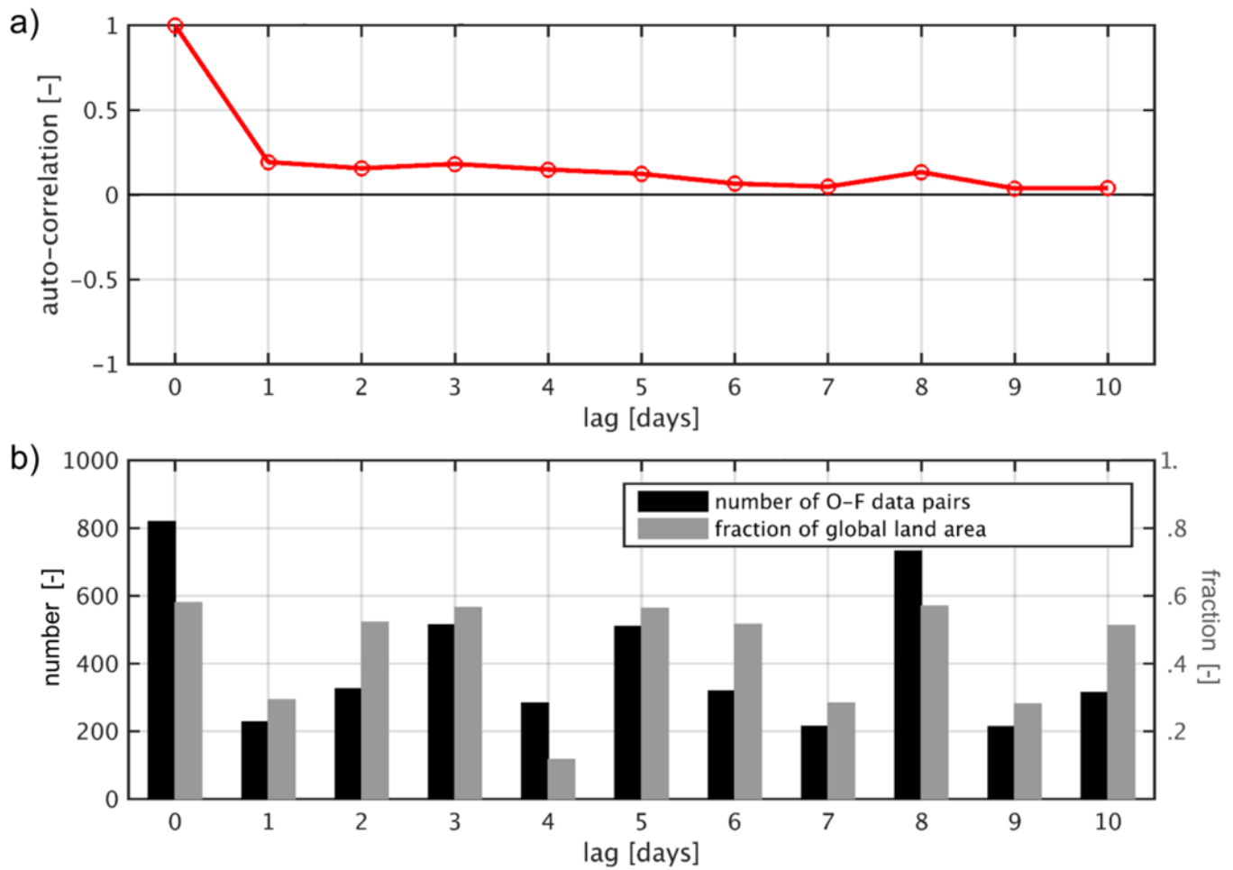
Fig. 8. (a) Spatially averaged, lagged sample auto-correlation of the O-F Tb residuals. (b) Average number of O-F data pairs at each grid cell (black; left axis) and fractional area coverage (gray; right axis) contributing to the sample auto-correlation values.
