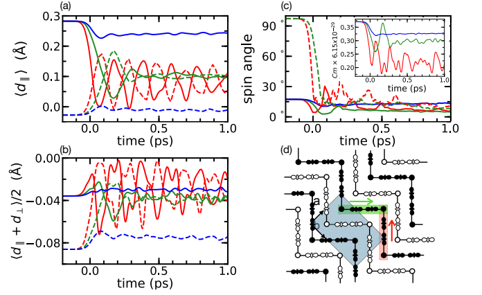
FIG. 3. Dissipation of the excited-electrons energy into the octahedral phonon modes and t_{2g} -spins. a): O-O bond expansions d_{||} (see Figure 1c) along the local trimer axes around \text{Mn}^{3+} (solid-lines), \text{Mn}^{4+} I (dashed-lines). b): average O-O bond expansion d_{||ab} = \langle \frac{d_{||} + d_{\perp}}{2} \rangle , around \text{Mn}^{4+} II (solid-lines) and \text{Mn}^{4+} III sites (dashed-lines). c): Evolution of the average intra-trimer spin angles (solid-lines) and inter-trimer spin angle along the direction of trimer (thick-lines). The inset shows evolution of average local dipole moment P_t = \langle \sum_i^5 \rho_i \vec{r}_i \rangle of tetramer units, indicated in red and green in panel d. The colored lines refer to the increasing intensities with 0.53 mJ/cm 2 (blue), 1.04 mJ/cm 2 (green) and 3.05 mJ/cm 2 (red). d): Photo-induced collinear SO in the ab -plane. Spin-up (spin-down) sites are indicated by white (black). The ab planes are antiferromagnetically coupled in \vec{c} direction.
