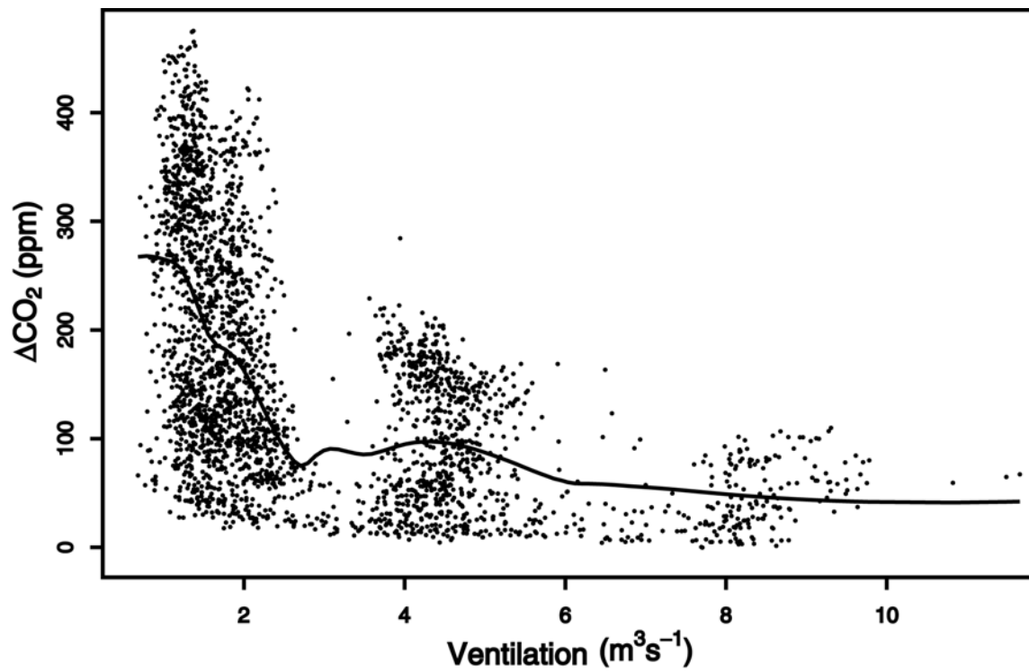
Figure 2. Indoor minus outdoor carbon dioxide concentrations plotted versus ventilation rates.
