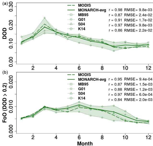
Figure 7. Globally averaged monthly global DOD_{\text{coarse}} (a) and FoO of DOD > 0.2 (b) for MODIS (dashed green line) and MONARCH ( DOD_{\text{coarse}} all-sky co-located with MODIS observations) (green solid line). The shading indicates the range of DOD_{\text{coarse}} across the four MONARCH experiments, which are also shown. Pearson correlation coefficients ( r ) and RMSE are given in the figure for both the experimental average as well as the individual runs.
