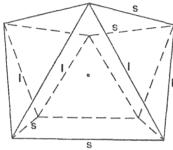
Square Antiprism D_{4d}
