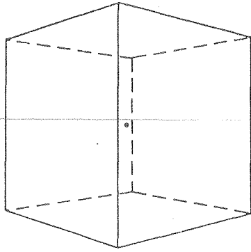
Cube O_h
