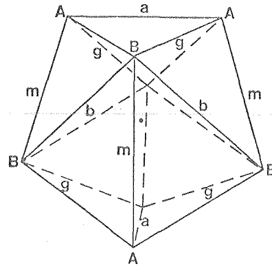
Dodecahedron D_{2d}
