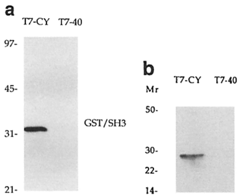
Figure 5. The cytoplasmic tail of CD2 binds directly to p56 lck . (a) T7-CY (lane 1) and T7-40 (lane 2) purified fusion proteins were immobilized onto anti-T7 mAb coupled to Sepharose bound rabbit anti-mouse antiserum and used to affinity precipitate 0.5 \mu g of GST/SH3 fusion protein in 1% NP-40 lysis buffer. The precipitates were washed three times in lysis buffer, eluted with Laemmli sample buffer, separated by SDS-PAGE, and immunoblotted with anti-GST antiserum. The presence of equimolar amounts of T7-CY and T7-40 was confirmed by immunoblotting with anti-T7 mAb (data not shown). (b) To equimolar amounts of T7-CY and T7-40 fusion protein, Sepharose bound GST/p56 lck SH3 was added and incubated for 1.5 h. The GST fusion protein was eluted in 10 mM glutathione, and the affinity precipitations were separated by SDS-PAGE and immunoblotted with anti-T7 mAb. Molecular masses are indicated on the left. Each figure is representative of at least three independent experiments.
