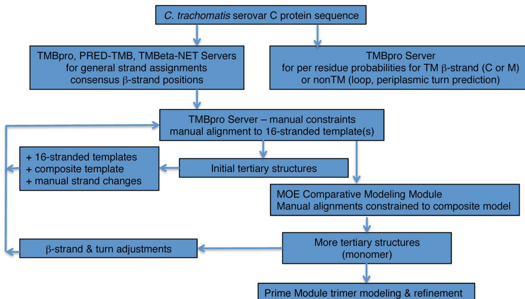
Figure 6. MOMP model construction flowchart.
