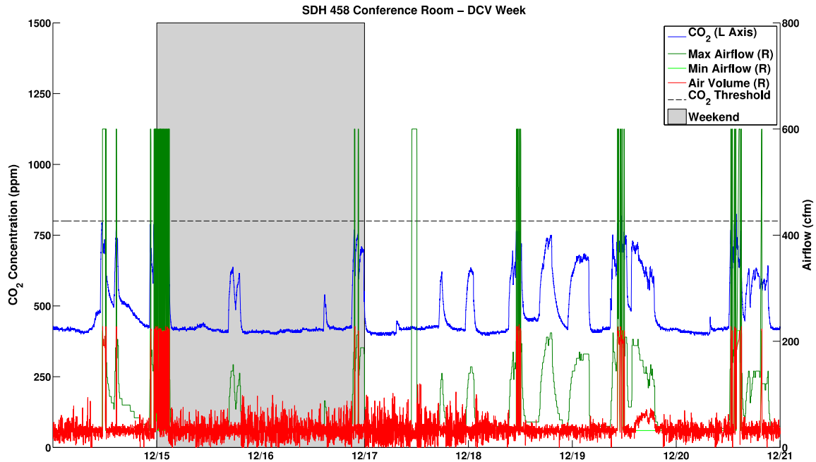
Figure 7. Operation of a conference room ventilation system with a demand-controlled ventilation strategy. Source: Taneja, 2013.
