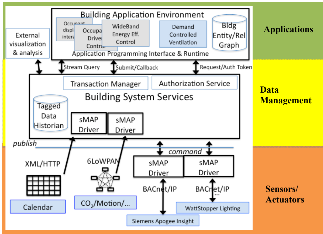
Figure 2. Building Operating System Services (BOSS): An open, layered distributed structure to bring advanced control and integrated operation into existing and new building stock. Note that in this instance BOSS is an overlay on the Siemens Apogee system and the WattStopper Lighting system, which are vertically integrated stacks. Source: adapted from Taneja et al. 2013.
