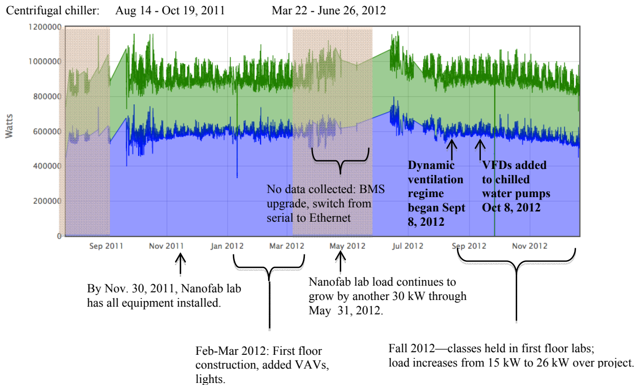
Figure 3. Whole building electrical load of Sutardja Dai Hall from May 22, 2011 to Dec 31, 2012 (MSA upper/green, MSB lower/blue) Source: Peffer 2012.
