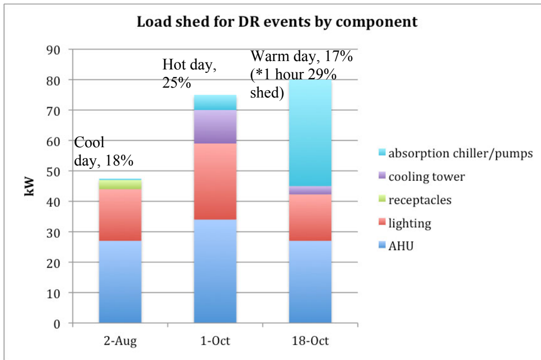
Figure 8. Summary of load shed for DR event days. Source: Auslander et al 2013.
