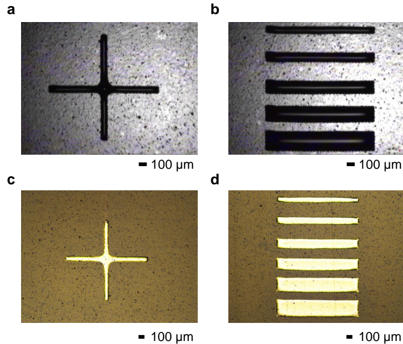
Figure 6.3. Printing resolution of the printed gold ink on the plasma treated Kapton ® PI substrate. (a, b) Printed cross and lines with increasing width. The cross and the top line in b are printed by placing two horizontal lines spaced 30\ \mu\text{m} apart, which yields 70\ \mu\text{m} minimum linewidth. While it is possible to use lines that are single-drop wide, two-drops wide lines are much more reproducible and reliable. Lines 2 - 5 (from the top) in b are 3 - 6 drops wide. (c, d) Microscope images of the sintered cross and lines with increasing width. Sintered shapes demonstrate <5\% shrinkage.
