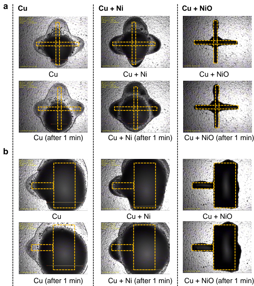
Figure 6.17. Nanoparticle ink wetting and spreading tests on different metallic surfaces. (a) 1\text{mm} \times 1\text{mm} printed cross and (b) 1\text{mm} long and 500\ \mu\text{m} wide printed tab on different metallic surfaces. The yellow dotted lines show the intended feature shape. In both (a) and (b), the top panel shows feature definition right after printing, while the bottom panel shows feature definition 1 min after printing. The first column in (a) and (b) shows printing on plated copper. The second column in (a) and (b) shows ink spreading on a nickel on copper surface. After a bake at 190\ ^\circ\text{C} for 30 min in air, an oxide layer is formed on the top of the nickel surface which restricts ink spreading to the metal features. The third column shows printed ink on this oxide surface. The pattern fidelity of printed features on the oxidized surface demonstrates significant improvement over the bare nickel on copper surface.
