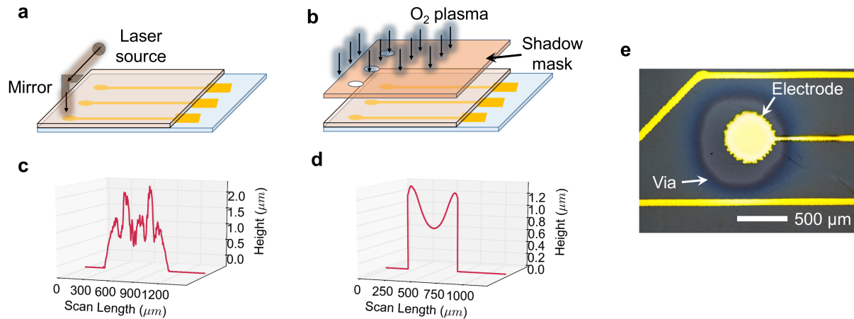
Figure 2.3. Methods for removing the dielectric layer (Cytob) from the electrodes. (a) Laser drilling to open via through the dielectric layer. (b) O_2 plasma etching using a shadow mask to selectively etch the dielectric layer. The surface profile of an electrode after (c) laser drilling and (d) plasma etching. (e) Micrograph of an electrode after plasma etching - etched area encircled by a dark Cytob layer, which is clearly visible; also the exposed electrode is shown.
