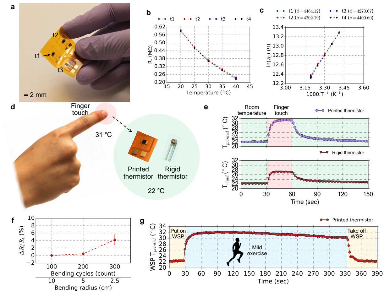
Figure 6.5. Characterization and dynamic testing of the stencil-printed thermistors. (a) Photograph of stencil-printed thermistors composed of NiO nanoparticles and PSBR binder on Kapton® PI substrate. The four thermistors are labeled t1, t2, t3, and t4. (b) Resistance vs. temperature plot for the thermistors. (c) \beta plot of the printed thermistors. (d) Characterization of the dynamic response of the printed thermistor. The printed thermistor and a commercial rigid thermistor are used to study the dynamic response. Both thermistors are touched with an index finger to record the change in temperature (22 to 31 °C). (e) The top panel shows the temperature read by the flexible thermistor and the bottom panel shows the temperature read by the rigid device. At normal condition (green), both thermistors show 22 °C, after touching the thermistors (red), the resistance drops due to the rise in temperature. As a result, the printed thermistor show 31 °C, and the rigid thermistor show 27 °C. (f) Durability testing of the printed thermistors. Bending radii of 10, 5, and 2.5 cm are used, and the thermistors are subjected to 100 bending cycles at every bending radius. The room temperature resistance of the thermistors roughly changed by 0, 0.5, and 4%, respectively (the error bars represent data collected from 8 devices). (g) Real-time temperature monitoring using the thermistor. The thermistor accurately measured skin temperature of 30 - 32 °C during the exercise (blue overlay).
